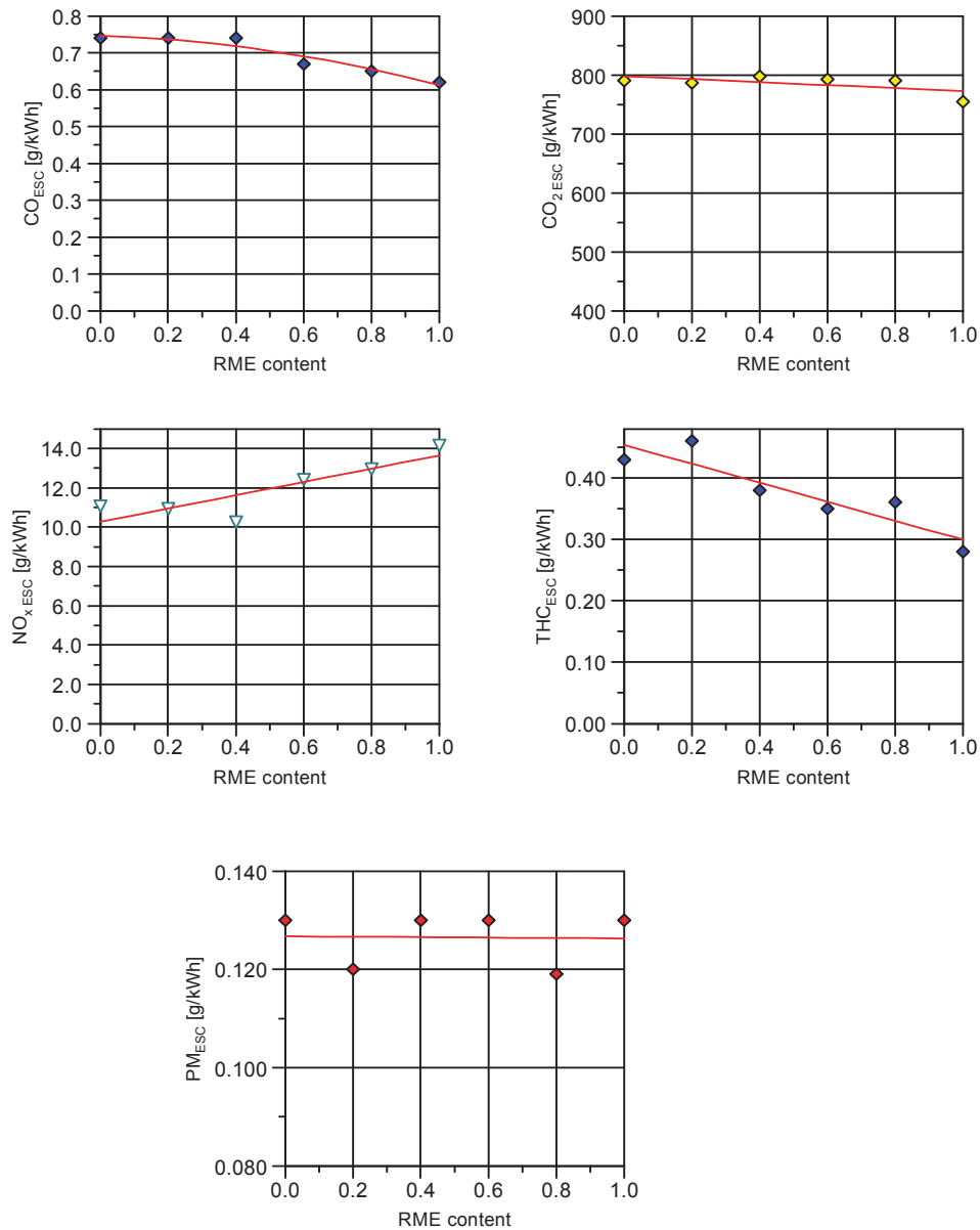
Fig. 1. Specific emission In European Steady Cycle (ESC) versus RME content in diesel oil
