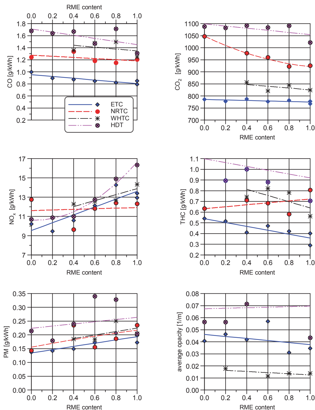
Fig. 2. Specific emissions in different transient cycles versus RME content in diesel oil
