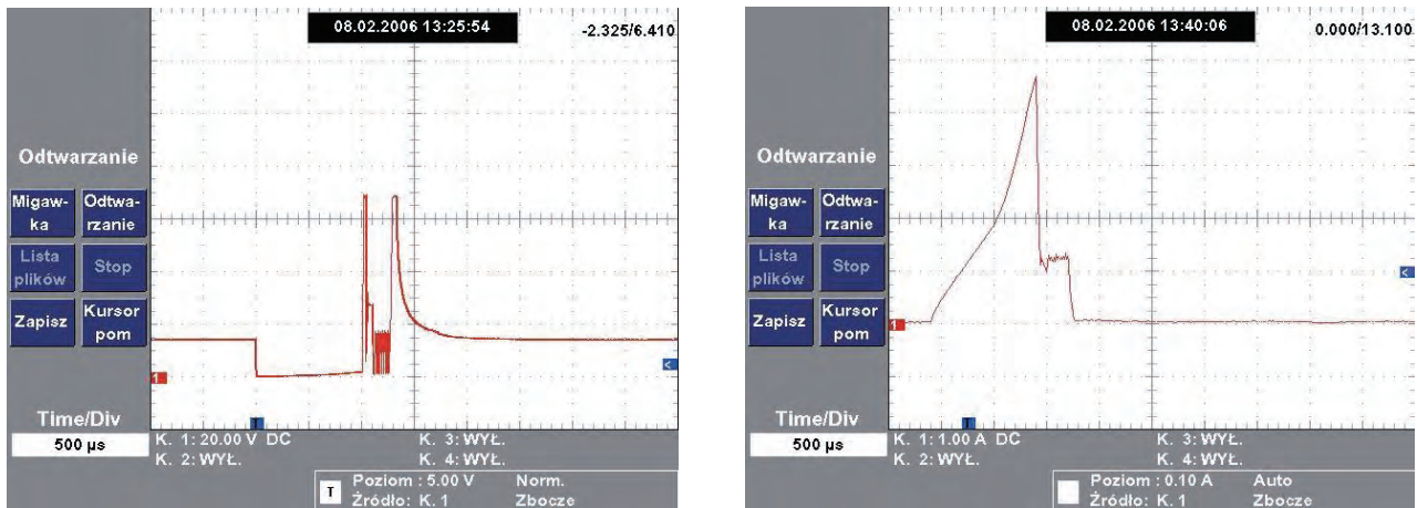
Fig. 6. The view of voltage (left) and current (right) which control the opening of the petrol injector needle. After the first needle raising pulse, the controller starts to time the voltage with hold the raised needle for injection period, which allows to reduce current from the engine controller power output. This operation is completed in engine even several dozen times a second (total injection time on idle run approx. 1.4 ms). The course of curves allows the skilled analyst for assessment of injector technical condition without any other special instruments (drawing and measurement – Piotr Stryjek)
