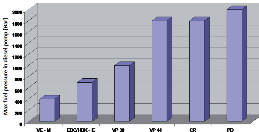
Fig. 3. The increase of maximum pressure in injecting systems – pump designations by BOSCH company types for car: VE-M – VP44 – distributor injection pump, CR – common rail, PD – fuel injection unit VW group (fig. Piotr Stryjek)
