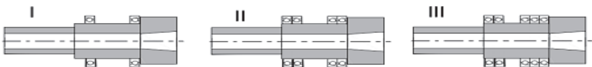
Fig. 9. Bearing distance effect on spindle shaft static stiffness
