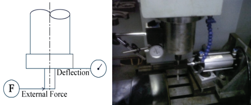
Fig. 3. Experimental setup for model validation
