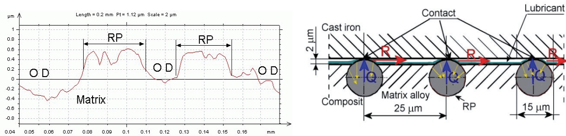
Fig. 1. 2D-roughness profile of composite piston skirt (a) and model of composite piston/cast iron cylinder liner contact: OD- oil depot, RP – reinforcing particle, R- friction force, Q – heat generated by friction
