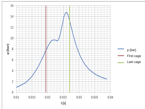
Fig. 6. High-speed waveforms of pressure in combustion chamber as a function of burning time: CR: 6:1, IT=30° CABTDC
