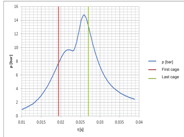
Fig. 8. High-speed waveforms of pressure in combustion chamber as a function of burning time: CR= 8:1; IT= 40° BTDC
