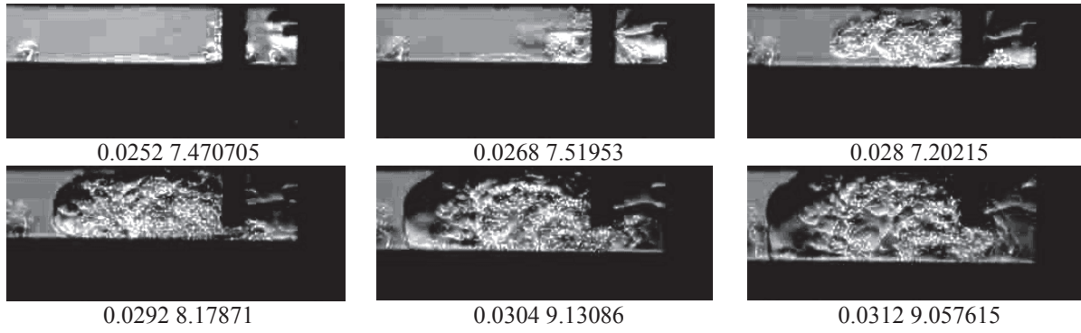
Fig. 5. Combustion process development in combustion chamber model: V_p=28\% , CR 6:1; IT=30° CABTDC
