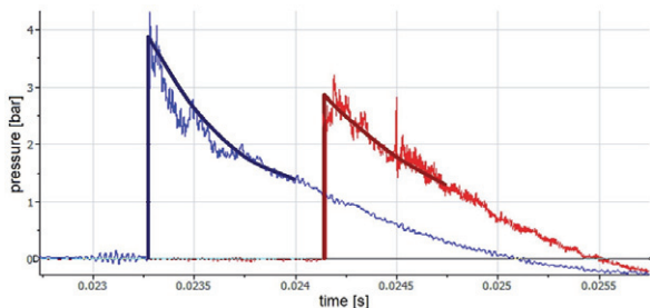
Fig. 8. Pressure Initiator – pressure 1 bar (test no. 32)
