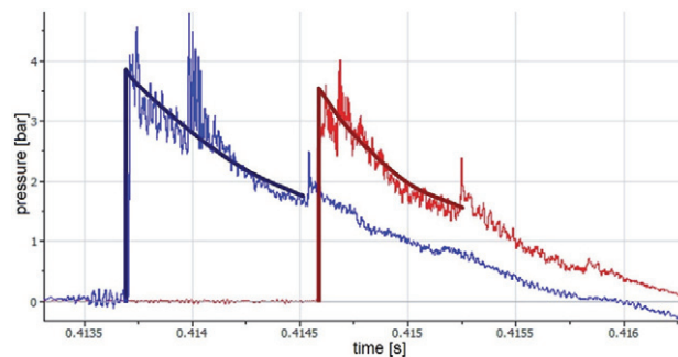
Fig. 5. Low Pressure Initiator (test no. 20)
