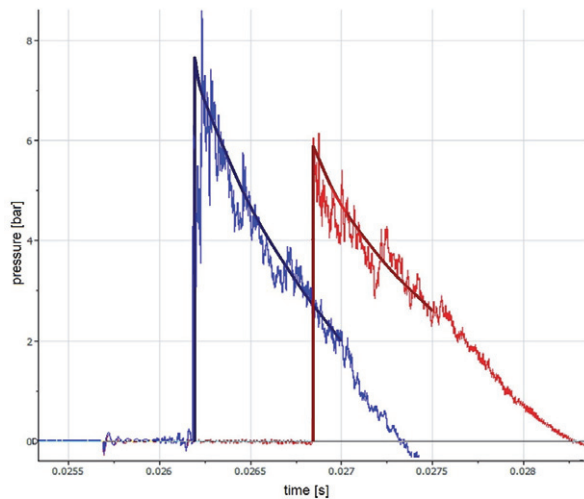
Fig. 6. High Pressure Initiator – pressure 3 bar (test no. 30a)
