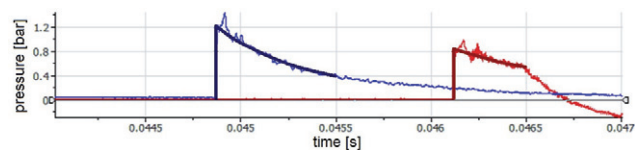
Fig. 9. Blank Ammunition Initiator (test no. 40b)
