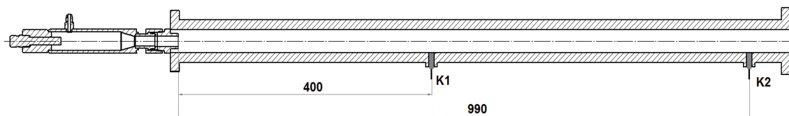
Fig. 4. The test stand scheme with measuring sensors (K1, K2) mounted
