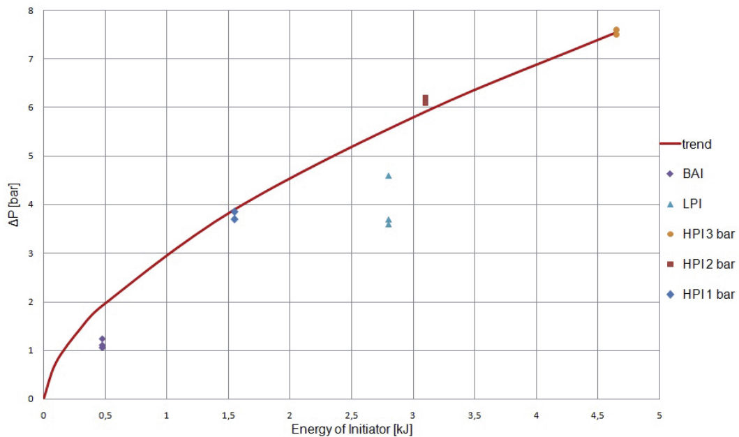
Fig. 6. Comparison of the effectiveness of tested initiators. \Delta P is a difference between pressure before and behind Shock wave
