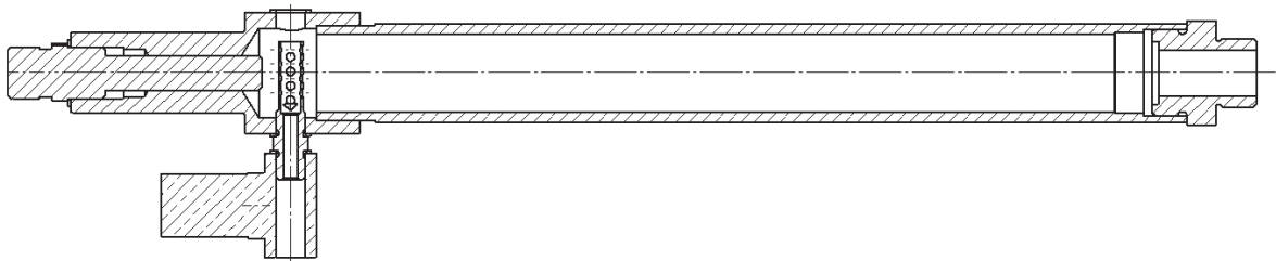
Fig. 2. Low Pressure Initiator
