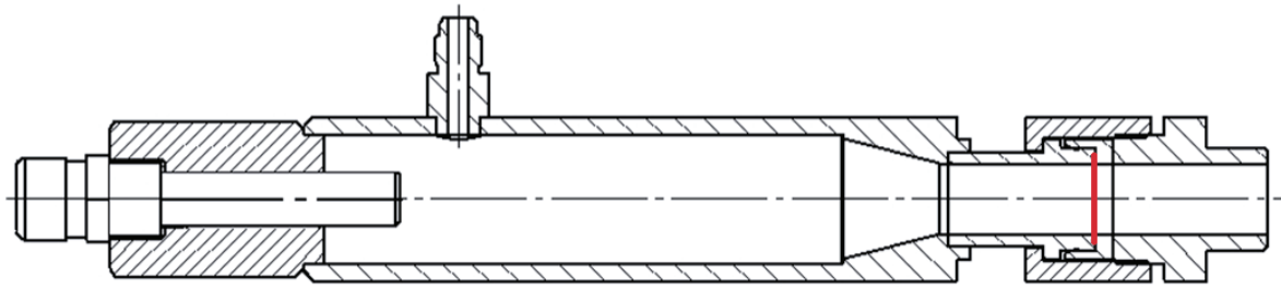
Fig. 1. High Pressure Initiator
