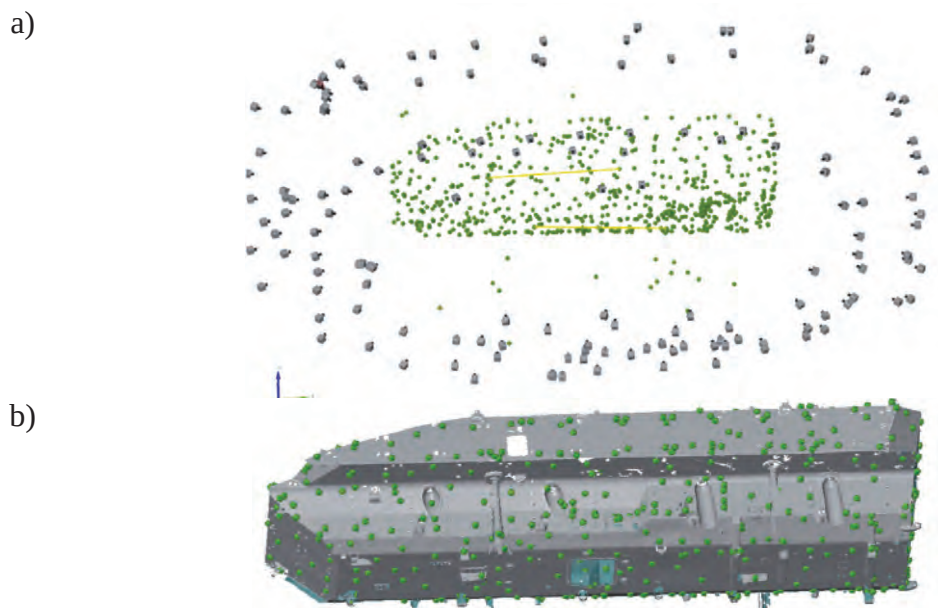
Fig. 2. Scanning stages: a) the image of markers placed on the surface and the positions of the camera around the vehicle, b) view of the vehicle body after scanning with markers
