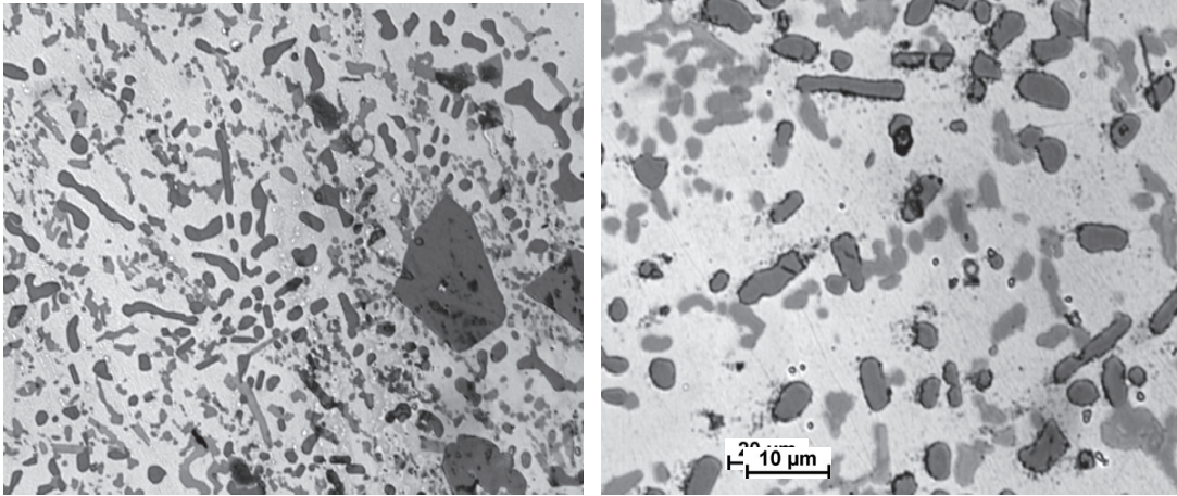
Fig. 3. Microstructure of the AlSi12Cu4Ni4Mg0.5CrMoWV silumin with additive of antimony after the solutioning at temperature 540°C.
