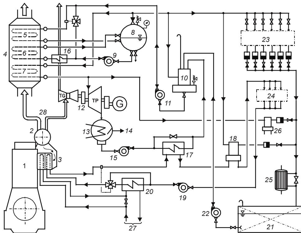
Fig. 6. Deep utilisation system utilising exhaust gases and scavenging air cooling heat: 1 – main engine; 2 – turbocharger; 3 – two-stage scavenging air cooler; 4 – waste heat boiler; 5 – internal feed; water heater; 6 – evaporator; 7 – steam superheater; 8 – steam drum; 9 – circulating pump; 10 – deaerator; 11 – waste heat boiler feed pump; 12 – combined turbine generator set (gas turbine, steam turbine, generator); 13 – condenser; 14 – vacuum system suction; 15 – condensate pump; 16 – fresh water generator water heater; 17 – condensate heater; 18 – steam water heater; 19 – heating water circulating pump; 20 – water heater; 21 – hot well; 22 – water refilling pump; 23 – heating steam receivers; 24 – heating water receivers; 25 – condensate cooler; 26 – final heavy fuel oil heater; 27 – low temperature cooling system connection; 28 – exhaust gases flow direction
