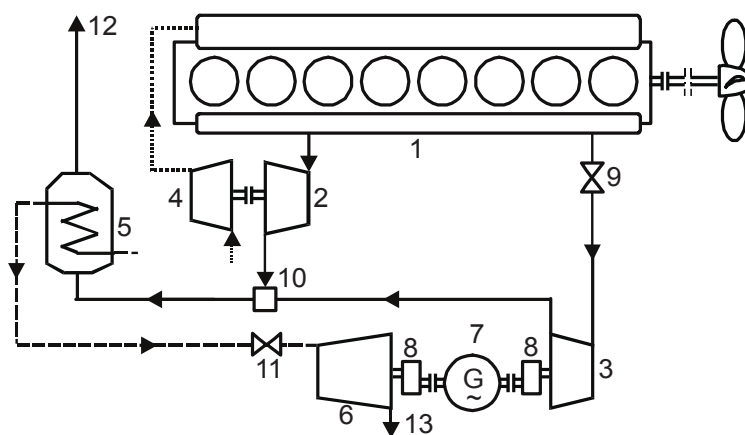
Fig. 1. Thermo Efficiency System: 1 – main engine; 2 – turbocharger turbine; 3 – power turbine; 4 – scavenging air compressor; 5 – waste heat boiler; 6 – steam turbine; 7 – generator; 8 – clutch; 9 – by-pass valve; 10 – mixing chamber; 11 – throttle valve; 12 – exhaust pipe; 13 – steam outlet
