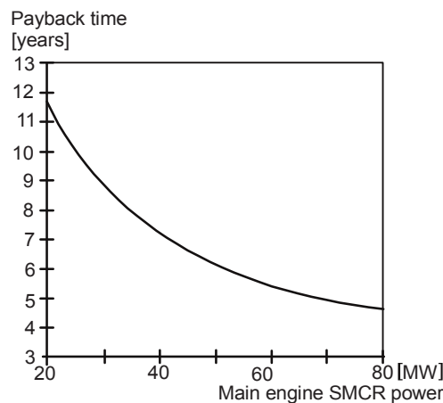
Fig. 8. Time of Thermo Efficiency System investment payback as a dependency on ship main engine power [4]. Normal service: 85% SMCR, service time 280 days/year, fuel consumption: 170 g/kWh
