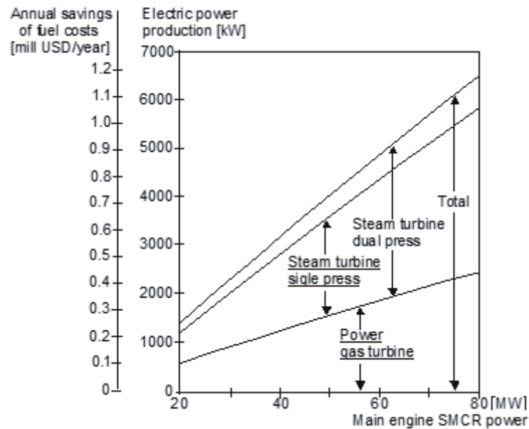
Fig. 7. Production of electric power and annual fuel costs savings of the Thermo Efficiency System as a dependency on ship main engine power [4]. Normal service: 85% SMCR, service time 280 days/year, fuel consumption: 170 g/kWh, fuel price: 160 USD/t
