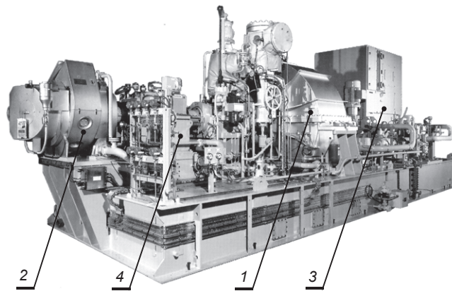
Fig. 3. Turbine generator set ABB type PTL: 1 – steam turbine; 2 – gas turbine; 3 – generator; 4 – reduction gear
