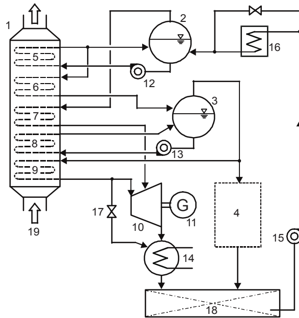
Fig. 5. Dual-pressure steam system: 1 – dual-pressure exhaust gas boiler; 2 – low pressure steam drum; 3 – high pressure steam drum; 4 – saturated steam receivers; 5 – low pressure evaporator; 6 – high pressure water heater; 7 – low pressure superheater; 8 – high pressure evaporator; 9 – high pressure superheater; 10 – dual pressure steam turbine; 11 – generator; 12 – low pressure circulating pump; 13 – high pressure circulating pump; 14 – condenser; 15 – feed pump; 16 – alternative feed water heater; 17 – dump valve; 18 – hot well; 19 – exhaust gas
