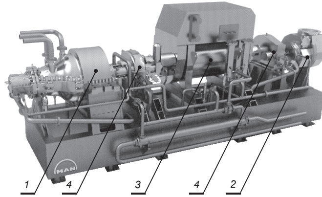
Fig. 2. Turbine generator set MAN type TES: 1 – steam turbine; 2 – gas turbine; 3 – generator; 4 – reduction gear
