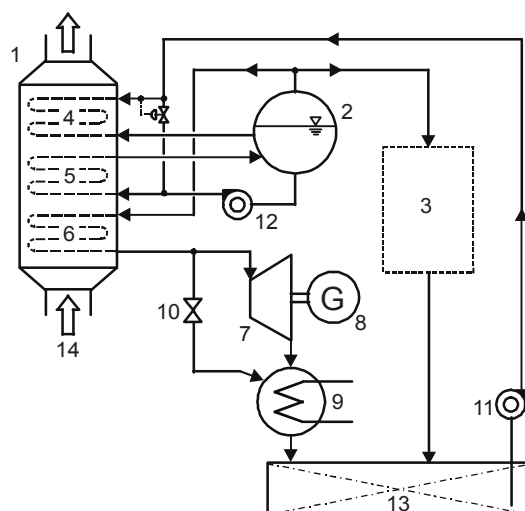
Fig. 4. Single-pressure steam system: 1 – single pressure exhaust gas boiler; 2 – steam drum; 3 – saturated steam receivers; 4 – feed water heater; 5 – evaporator; 6 – superheater; 7 – steam turbine; 8 – generator; 9 – condenser; 10 – dump valve; 11 – feed pump; 12 – circulating pump; 13 – hot well; 14 – exhaust gas
