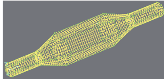
Fig. 3. Discretized model of the modified exhaust system [1]
