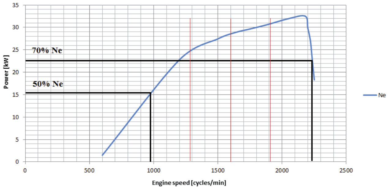
Fig. 6. Power output depending on the rot. speed of the crankshaft with marked measuring points ESC test [1]
