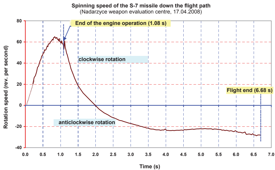
Fig. 11. Rotation speed variations for the S-7 missile during the flight
