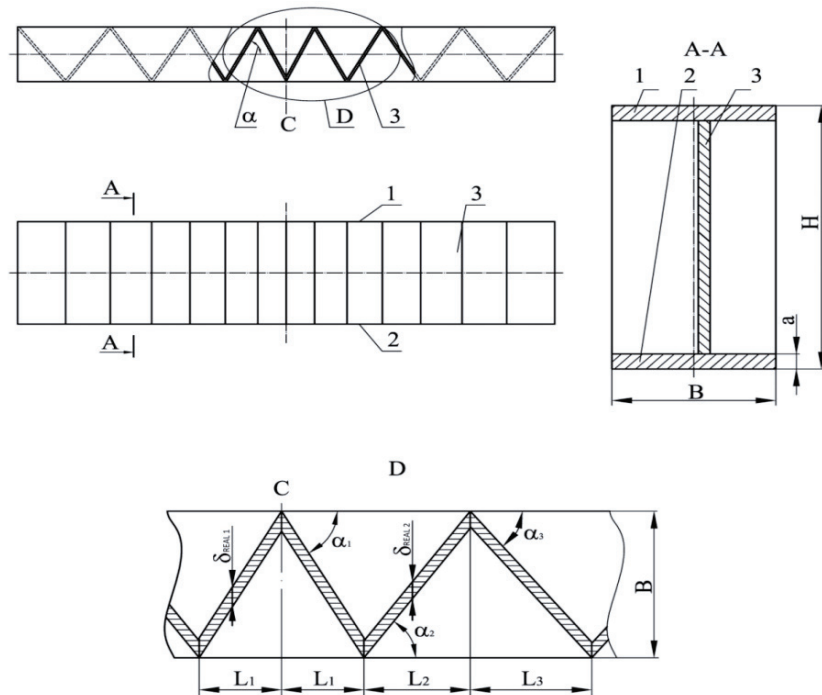
Fig. 4. Span beam [7, 8]
