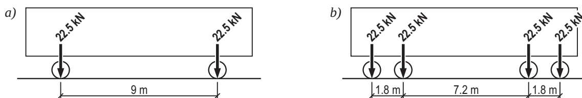
Fig. 3. Schemes of the considered wagons equipped with two single axles (a) and two 2-axle bogies (b)
