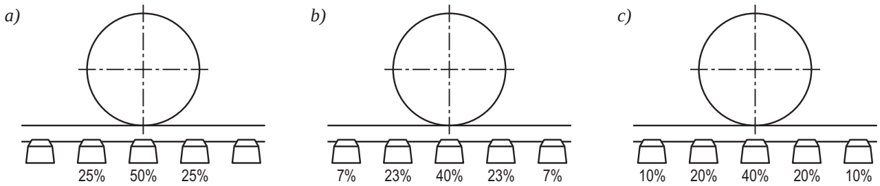
Fig. 1. Load distribution along successive sleepers: suggested by Awolaye (a), Watanabe (b), and the US Army Corps of Engineers (c) [1–3]
