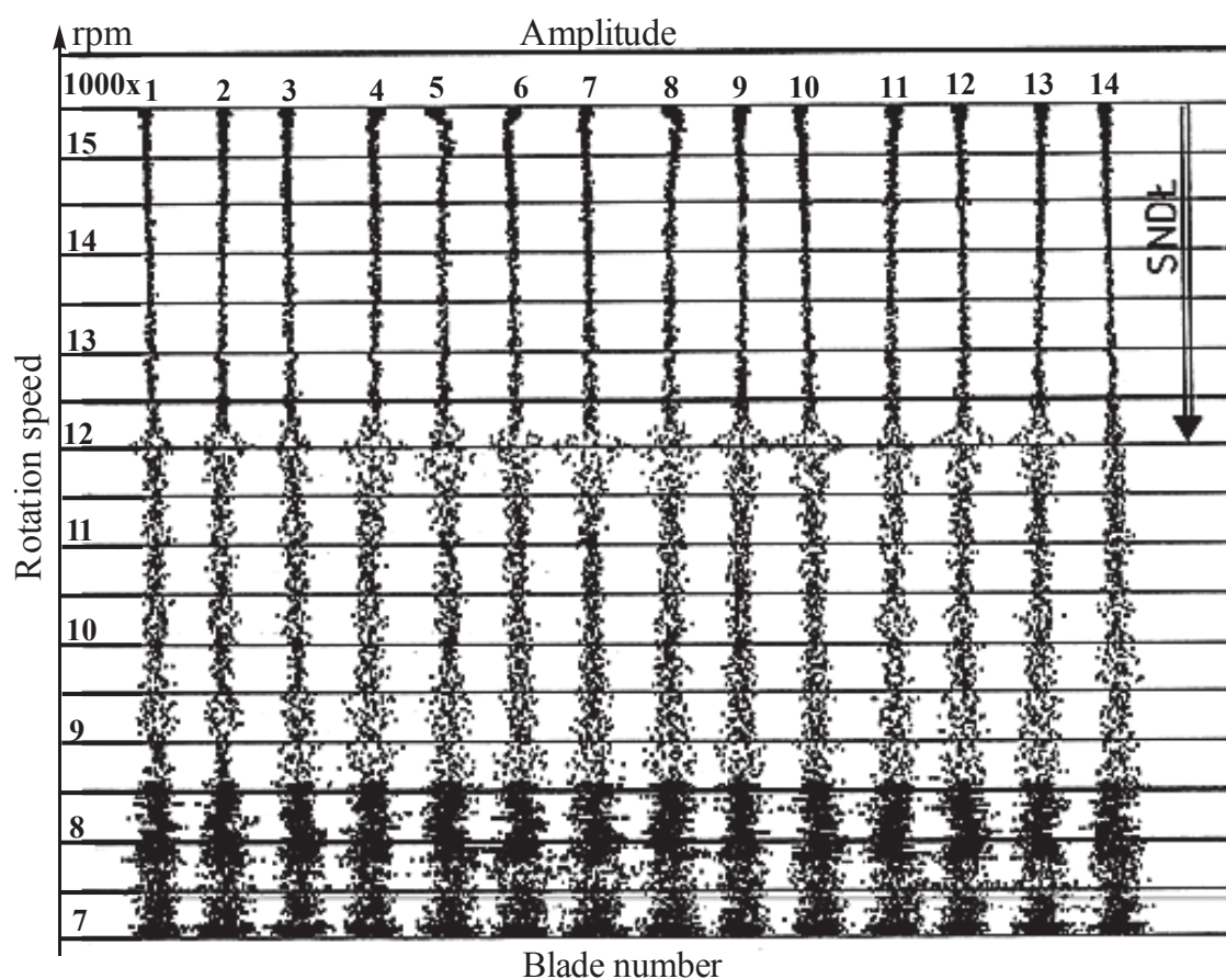
Fig. 15. Vibration amplitudes of compressor 1st stage rotor blades 1 and 14
