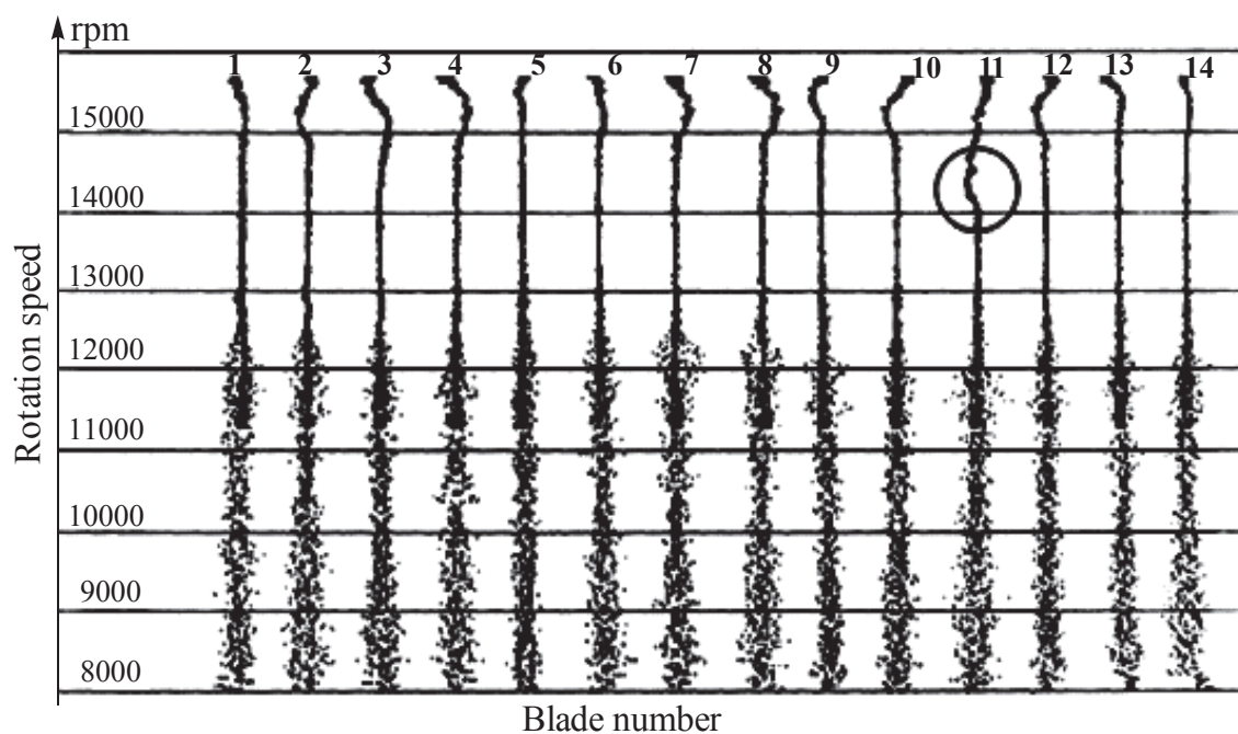
Fig. 14. Vibration amplitudes of compressor 1st stage rotor blades, with crack initiation in one of the rotor blades
