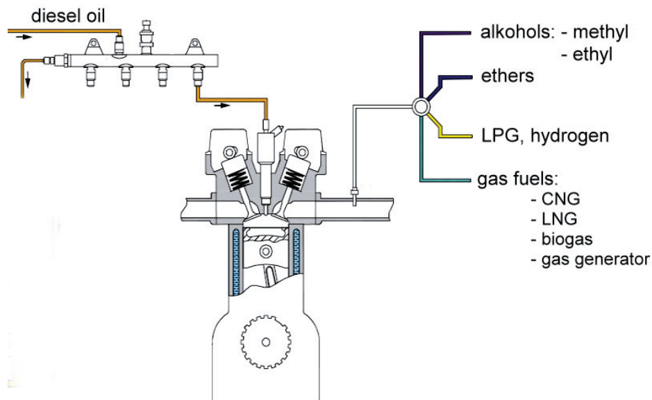
Fig. 1. Possibilities of dual fuel supply of compression ignition engine
