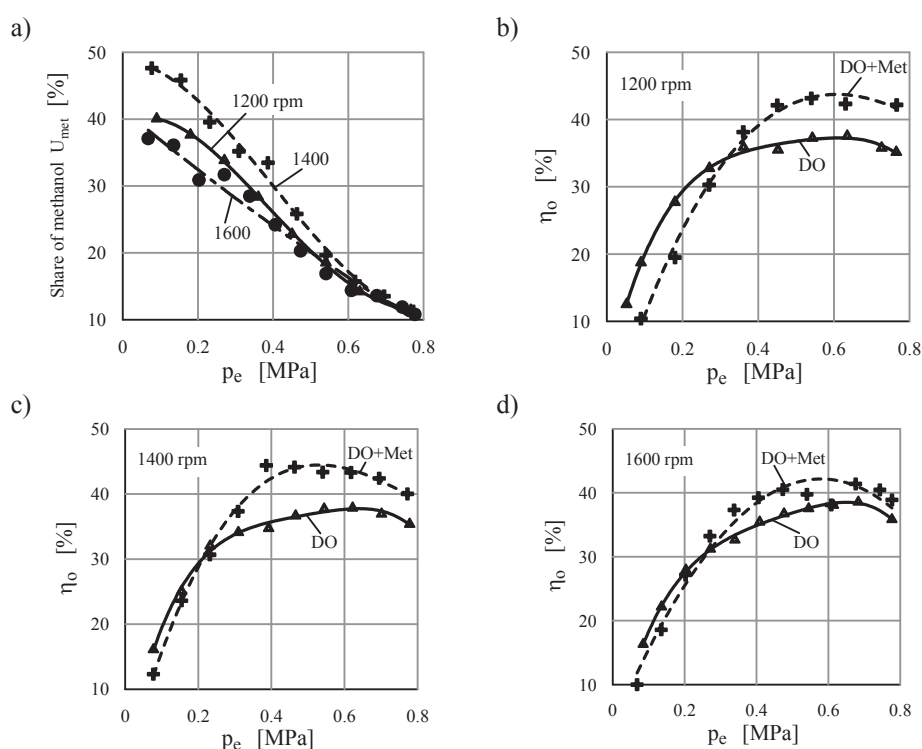
Fig. 5. Comparison of energetic fraction of the methanol and overall efficiency of the SW 680 engine fuelled with Diesel oil and run in dual fuel system – fuelled with Diesel oil and methanol: different rotational speeds
