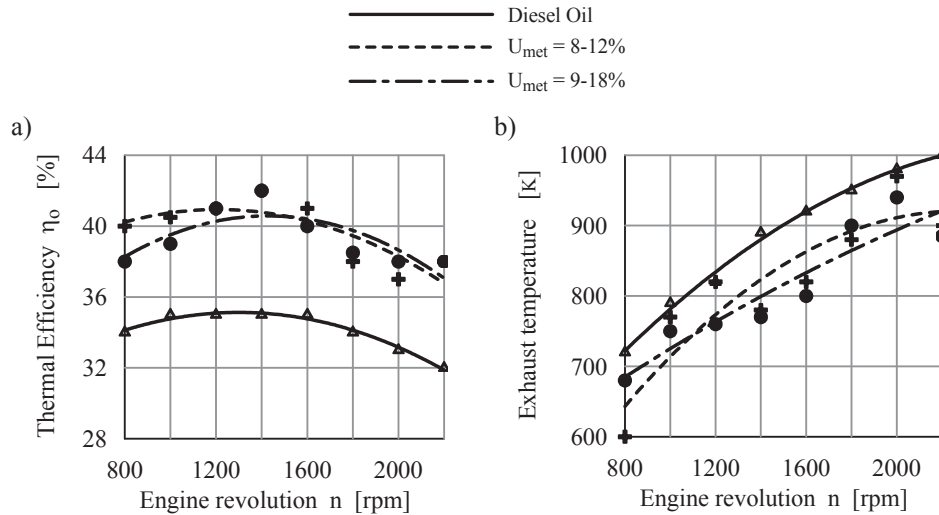
Fig. 2. Effect of rotational speed on overall efficiency and temperature of exhaust gases of the SW 680 engine operated on Diesel oil and run in dual fuel system, fuelled with Diesel oil and methanol: maximal engine load
