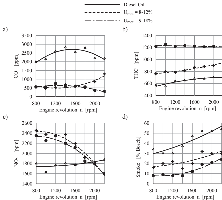
Fig. 3. Comparison of concentrations of exhaust gases components of the SW 680 engine fuelled with Diesel oil and methanol
