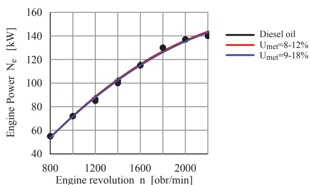
Fig. 4. Comparison of maximal power output of the SW 680 engine run in dual fuel system – fuelled with Diesel oil and methanol
