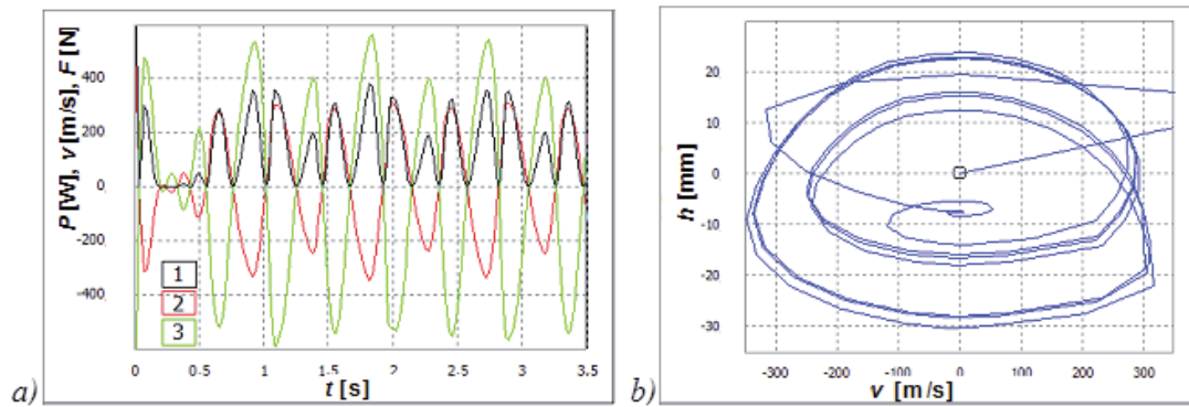
Fig. 8. Courses against time for: 1 – the power of generator in shock absorber, 2 – velocity of the rod the shock absorber, 3 – force generated in the shock absorber (a). Phase diagram displacement – velocity of the rod relative to the cylinder, the case of the wheel with steel rim (b)
