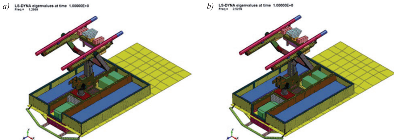
Fig. 6. Selected forms of own vibrations of the supporting structure of the container: a) the first form for the frequency f_1 = 1.3 Hz, b) the third form for the frequency f_2 = 2.52 Hz
