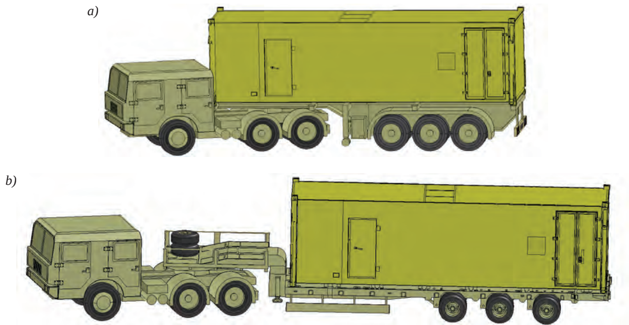
Fig. 6. A transport unit with a military saddle tractor: a) classic trailer by ZREMB, b) increased mobility trailer by Auto-Hit sp. z o.o.
