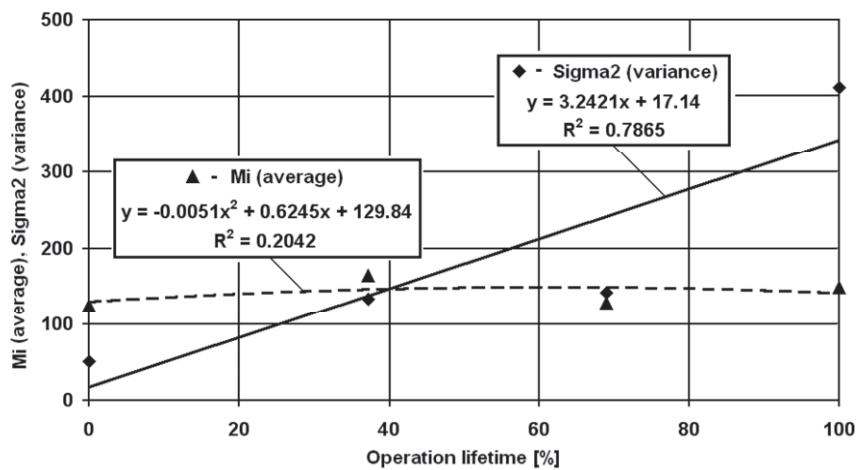
Fig. 8. Variations of the second order statistical parameters – Mi – average and \text{Sigma}^2 – variance
