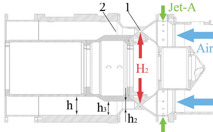
Fig. 9. Scheme of the chamber with three-part inner channel: 1 – detonation chamber inlet throat, 2 – detonation chamber, h – height of the channel adjusted to detonation cell size of Jet-A- O_2 mixture (50 mm), h_2 – height of the channel adjusted to detonation cell size of H_2 - O_2 mixture (20 mm), h_3 – height of the transfer passage between the wide and narrow part
