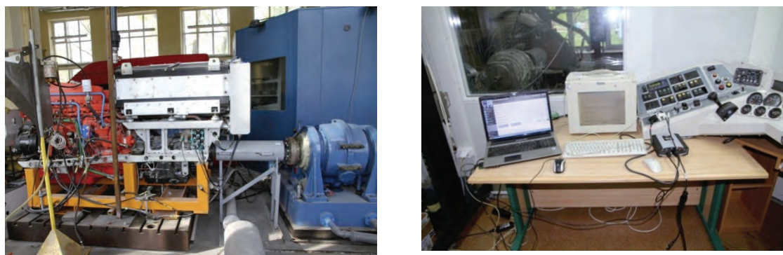
Fig. 2. Test stand for test drive units AMV Rosomak: a) the engine with the gearbox, in the back can see the control cabin, b) diagnostics device TEXA with computer and driver's console (Source: by authors)
