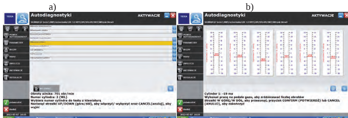
Fig. 6. The results of measurements: a) balance of cylinders, b) the deviation of fuel dose (Source: by authors)
