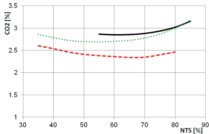
Fig. 12. \text{CO}_2 -concentration: — original injector (JET-A1), -- Conical-type injector No. 2 (LPG), .... multi-hole injector No. 5 (LPG)
