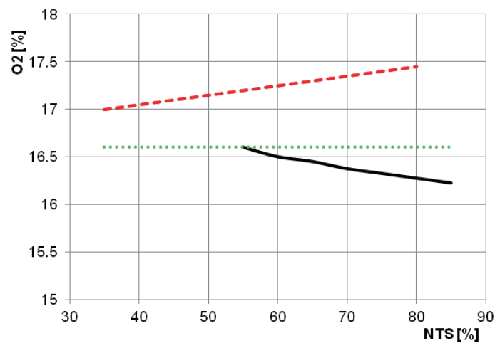
Fig. 13. \text{O}_2 -concentration: — original injector (JET-A1), -- Conical-type injector No. 2 (LPG), .... multi-hole injector No. 5 (LPG)
