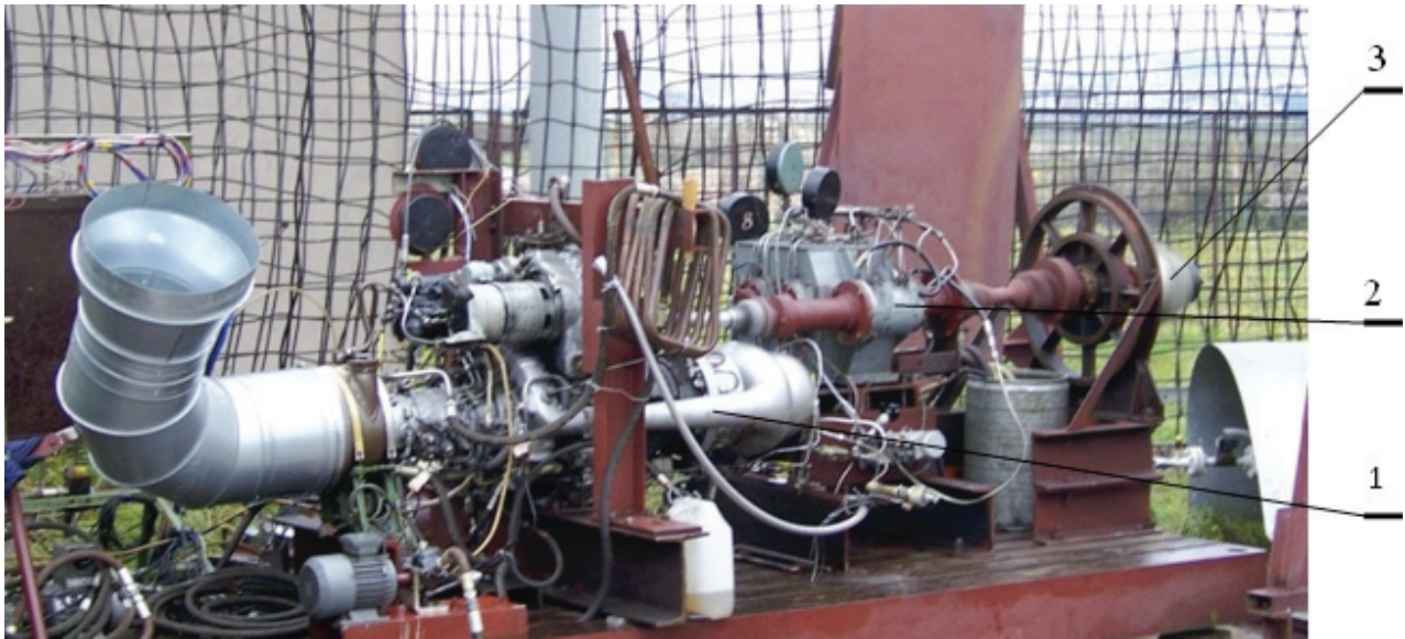
Fig. 1. View of test bench: 1 – GTD-350 engine, 2 – gear, 3 – propeller
