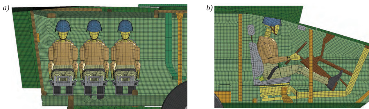
Fig. 1. The location of dummies inside a carrier: troops (a), driver (a)
