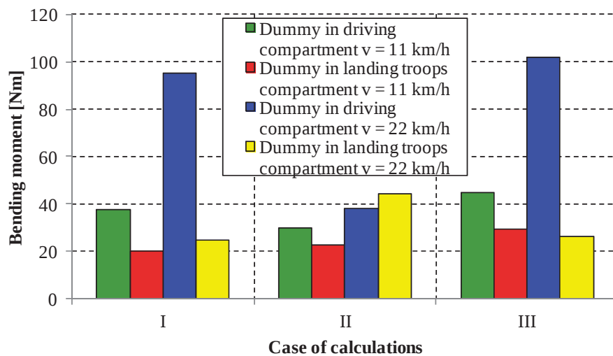
Fig. 8. The distribution of neck bending moment
