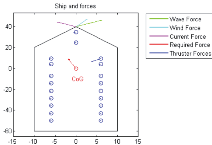
Fig. 3. The propulsion system with 20 thrusters need as a minimum only 12.2 MW of total power for required DP capability [11]
