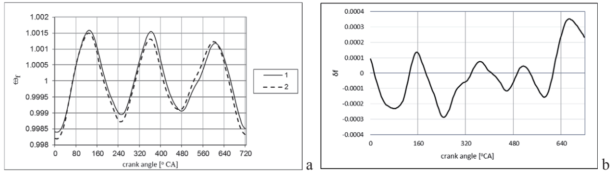
Fig. 2. Runs of relative angular speed of healthy engine (line 1) and faulty (line 2) – a, and related to that failure values of parameter \delta_f – b
