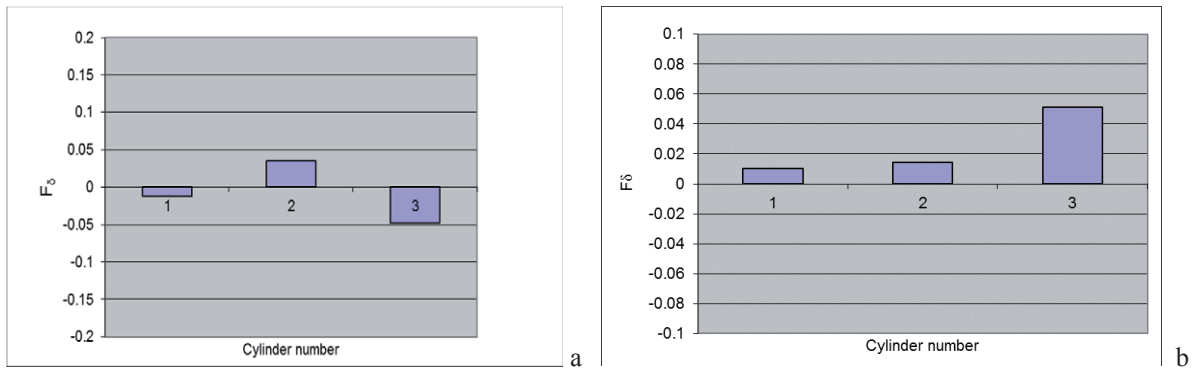
Fig. 8. Pattern of coefficient F_\delta "weak spring": a – load 150 kW, b – load 250 kW
