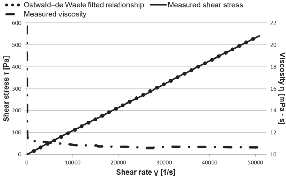
Fig. 1. Shear stress and viscosity vs. shear rate for Superol CC-40 at temperature t = 90^\circ\text{C} . K = 0.01147 \text{ Pa}\cdot\text{s}^n , n = 0.9932 , \eta_0 = 21.7 \text{ mPa}\cdot\text{s} , \eta_\infty = 10.6 \text{ mPa}\cdot\text{s}
