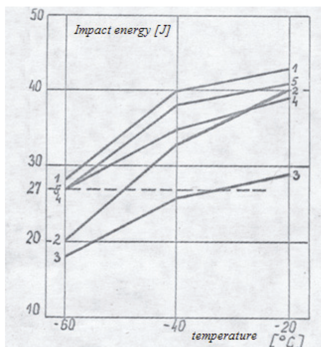
Fig. 4. KV impact energy at breaking welded joint samples made of S540Q steel. The places of notches cuts: 1 – native material, 2 – weld axis, 3 – transition zone, 4 – HAZ 2 mm from transition zone, 5 – SWC 5 mm from transition zone
