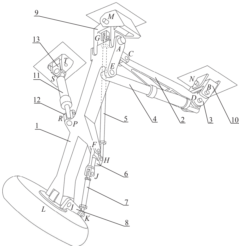
Fig. 1. The mechanism of the Lockheed F-104S Starfighter landing gear
