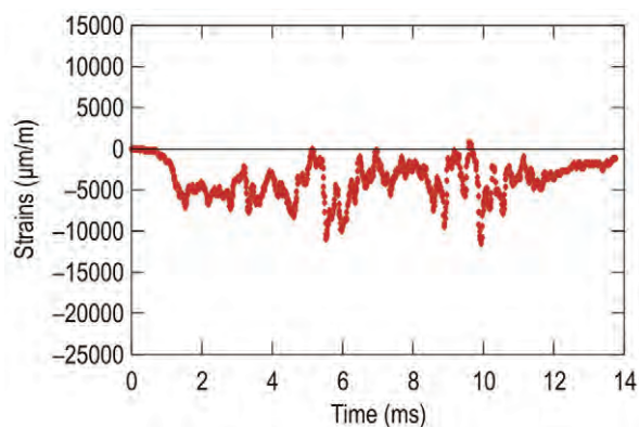
Fig. 7. Plot of \varepsilon - t for the measurement point “0”
