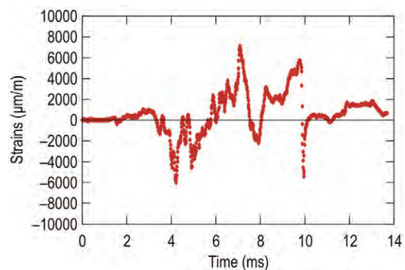
Fig. 11. Plot of \varepsilon - t for the measurement point “4”
