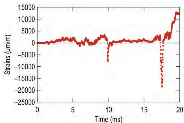
Fig. 12. Plot of \varepsilon - t for the measurement point “5”
