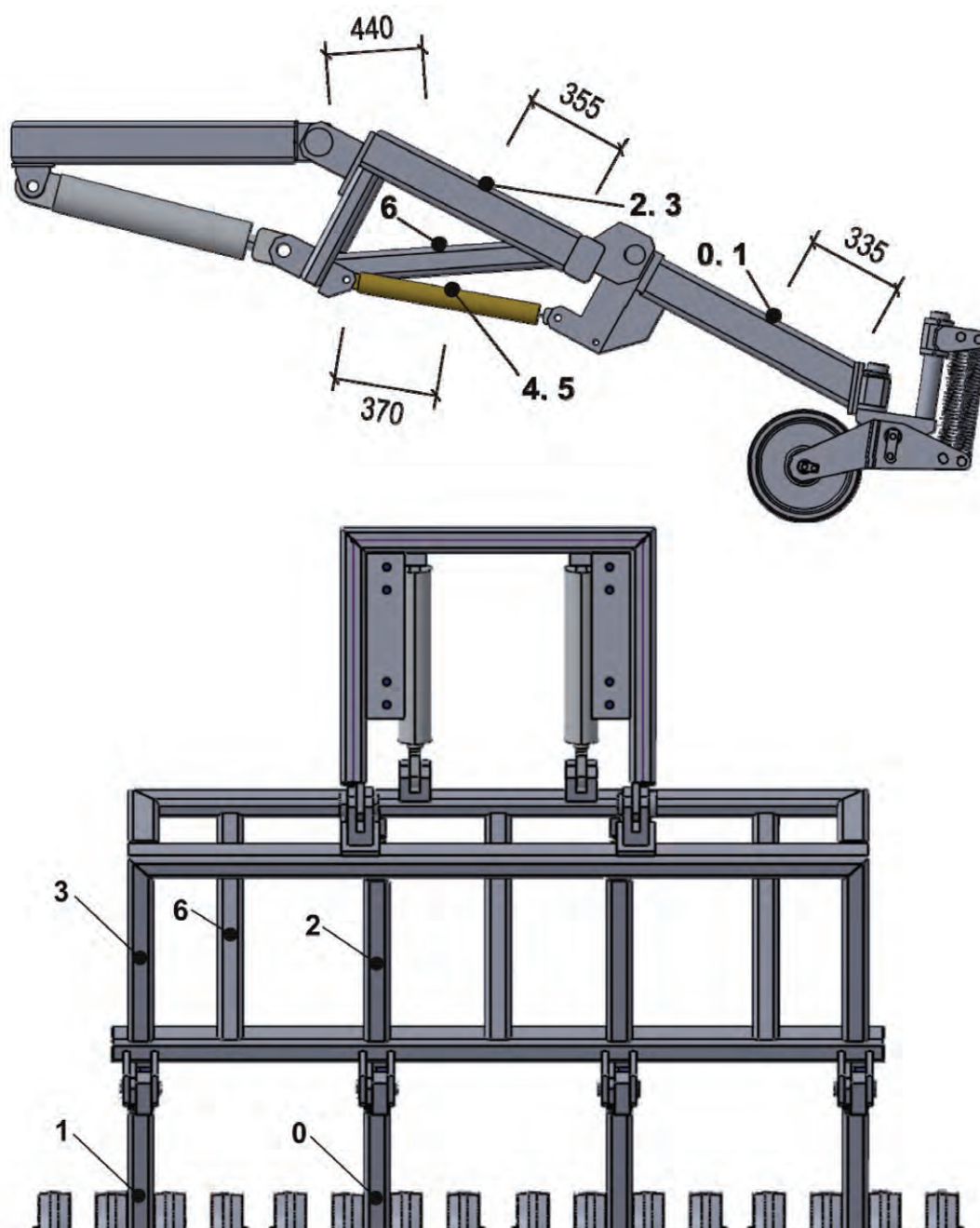
Fig. 1. Diagram of location of the measurement points – dimensions in (mm)
