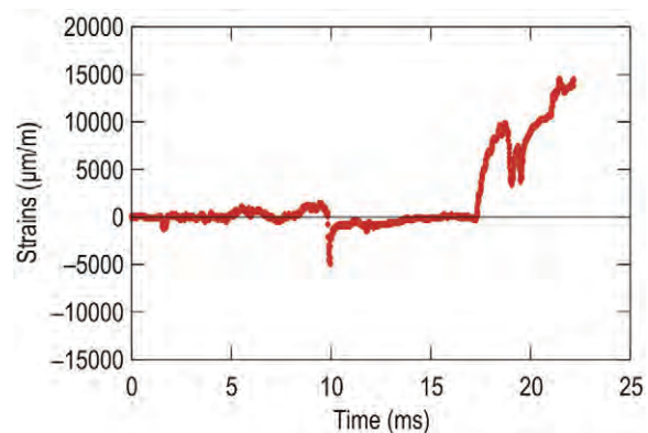
Fig. 9. Plot of \varepsilon - t for the measurement point “2”
