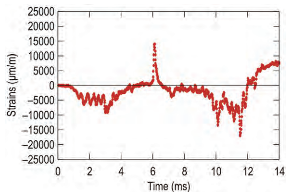
Fig. 8. Plot of \varepsilon - t for the measurement point “1”
