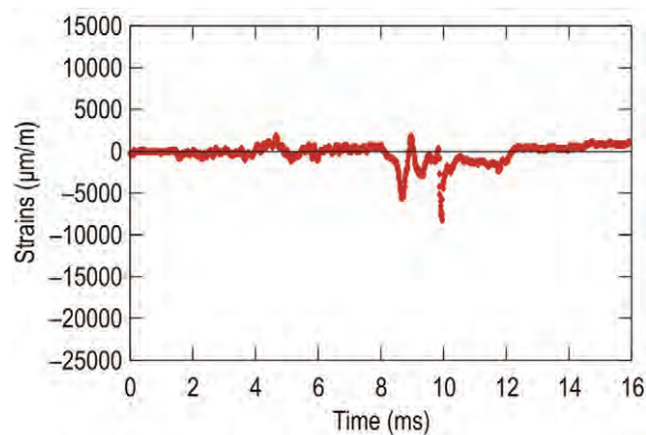
Fig. 13. Plot of \varepsilon - t for the measurement point “6”
