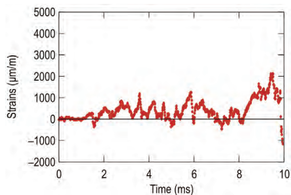
Fig. 10. Plot of \varepsilon - t for the measurement point “3”
