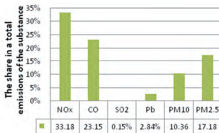
Fig. 2. The share of road transport in air pollution. Source: own work based on 0
