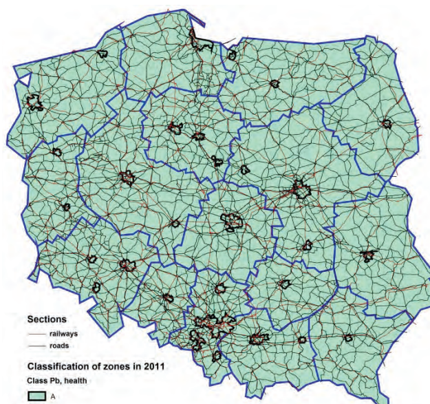
Fig. 8. Classification of zones in Poland for Pb in 2011 (criterion f_1 ). Source: printout from PTV VISUM based on [7]
