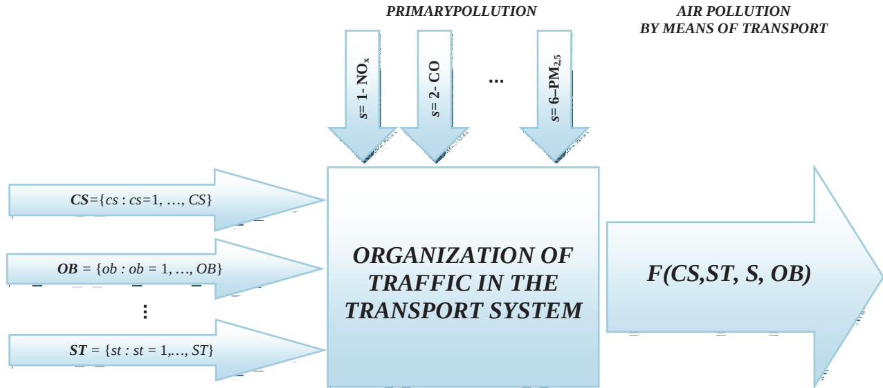
Fig. 4. Air pollution by means of transport. Source: own work
