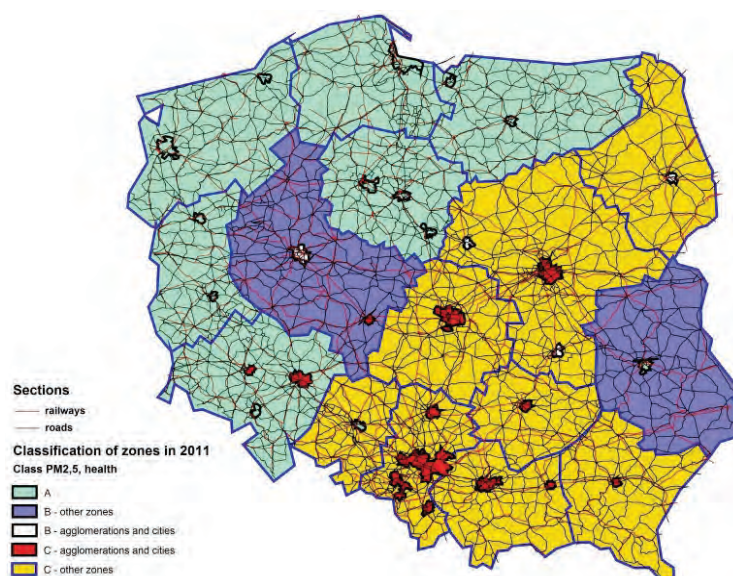
Fig. 12. Classification of zones in Poland for PM_{2.5} in 2011 (criterion f_1 ). Source: printout from PTV VISUM based on [7]
