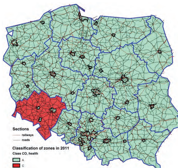
Fig. 7. Classification of zones in Poland for CO in 2011 (criterion f_1 ). Source: printout from PTV VISUM based on [7]
