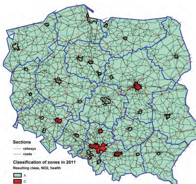
Fig. 5. Classification of zones in Poland for \text{NO}_2 in 2011 (criterion f_1 ). Source: printout from PTV VISUM based on [7]
