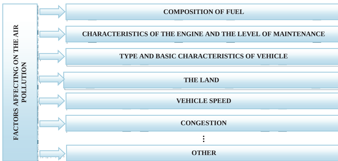
Fig. 1. Factors affecting the air pollution coming from the sphere of transport. Source: own work based on [4]
