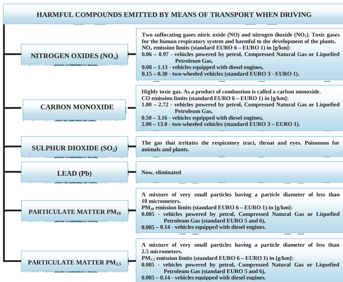
Fig. 3. Harmful compounds emitted by means of transport when driving. Source: own work based on [6, 11]
