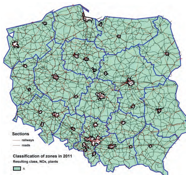
Fig. 6. Classification of zones in Poland for \text{NO}_x in 2011 (criterion f_2 ). Source: printout from PTV VISUM based on [7]
