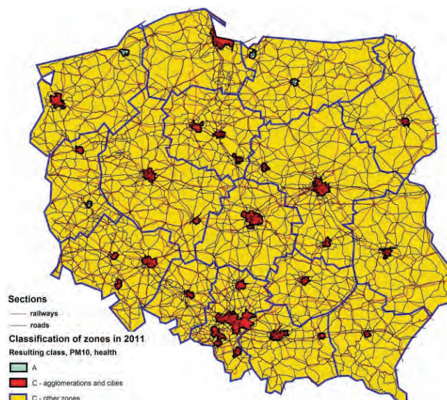
Fig. 11. Classification of zones in Poland for PM_{10} in 2011 (criterion f_1 ), source: printout from PTV VISUM based on [7]
