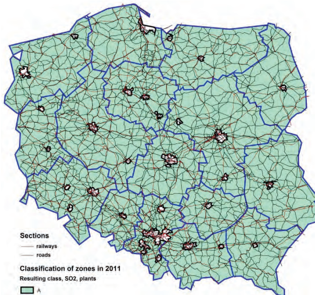
Fig. 10. Classification of zones in Poland for \text{SO}_2 in 2011 (criterion f_2 ). Source: printout from PTV VISUM based on [7]
