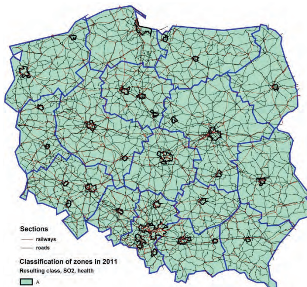
Fig. 9. Classification of zones in Poland for \text{SO}_2 in 2011 (criterion f_1 ). Source: printout from PTV VISUM based on [7]
