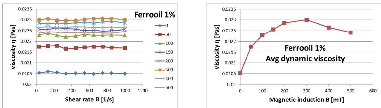
Fig. 1. The characteristics of dynamic viscosity of 1% ferro-oil and averaged values of dynamic versus shear rate changes from 0 to 1000\ s^{-1} and versus magnetic induction field B = 50, 100, 150, 200, 300, 400, and 500\ mT respectively
