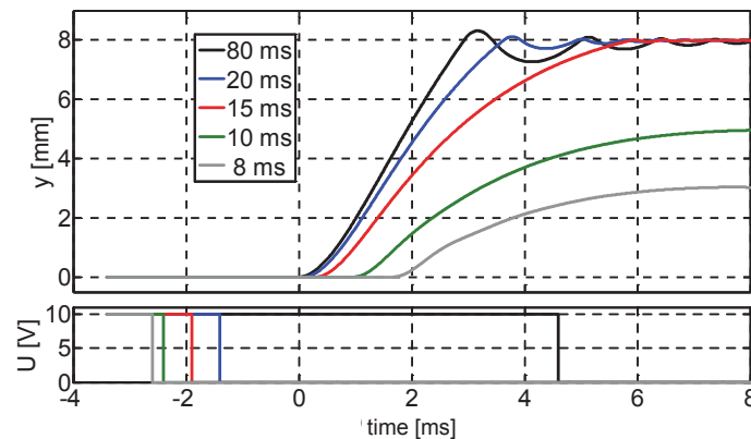
Fig. 11. The effect of control signal duration on valve lift
