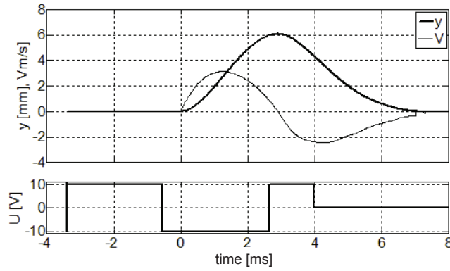
Fig. 8. Waveforms of: valve lift, valve speed and the control signal for a supply pressure of 10 MPa and engine speed 6000 rpm with valve braking
