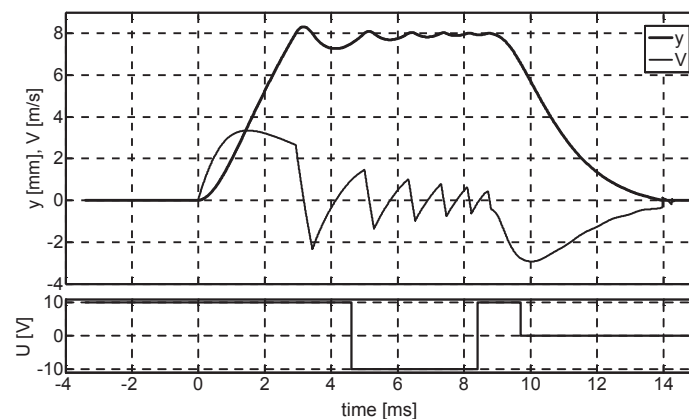
Fig. 5. Waveforms of: valve lift, valve speed and the control signal for a supply pressure of 10 MPa and engine speed 3000 rpm with valve braking
