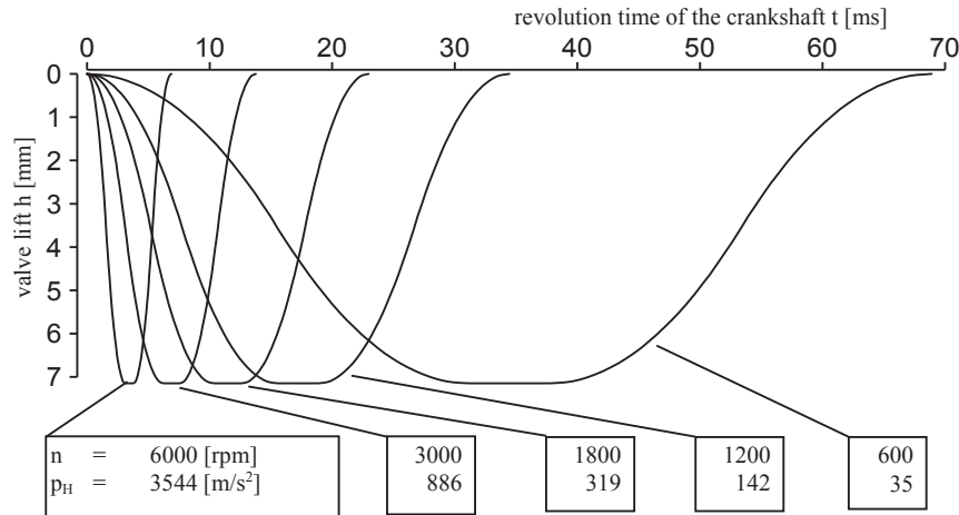
Fig. 1. Waveforms of valve lift driven by a harmonic cam, for engine speeds from 600 to 6000 rpm
