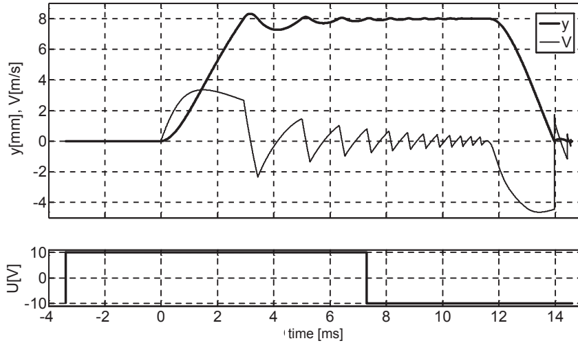
Fig. 6. Waveforms of: valve lift, valve speed and the control signal for a supply pressure of 10 MPa and engine speed 3000 rpm without valve braking
