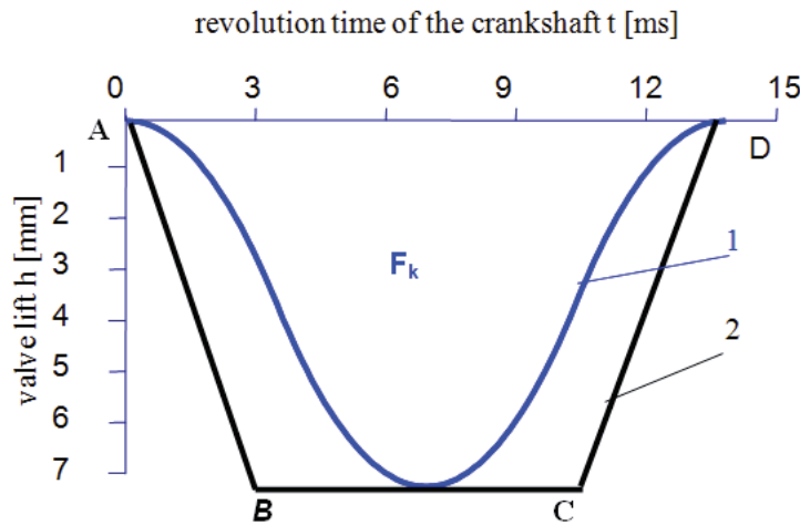
Fig. 2. Waveforms of valve lift for engine speeds 3000 rpm: 1 – the real waveform of valve lift mechanically driven by a harmonic cam, 2 – theoretic, desired waveform of valve lift hydraulically driven
