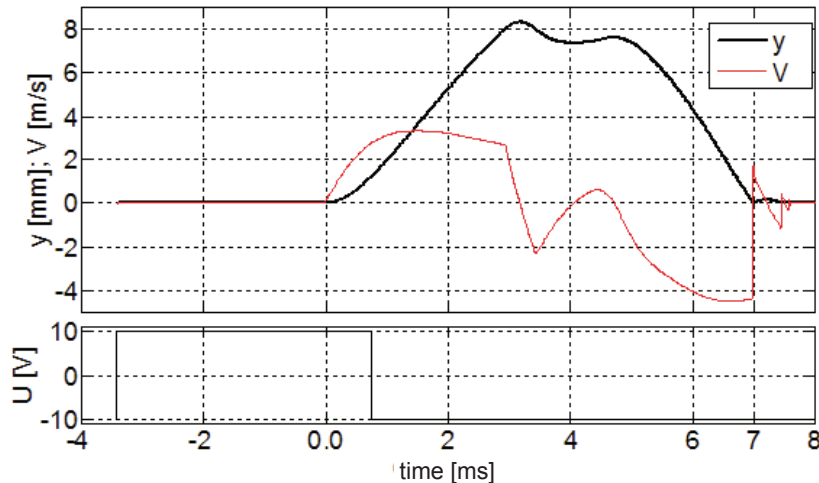
Fig. 7. Close to the theoretical waveforms of: valve lift, valve speed and the control signal for a supply pressure of 10 MPa and engine speed 6000 rpm without valve braking
