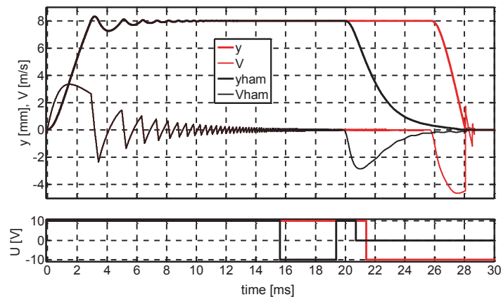
Fig. 10. Waveforms of: valve lift, valve speed and the control signal for a supply pressure of 14 MPa and duration of valve lift 28 ms (black lines-with valve braking, red lines-without valve braking)
