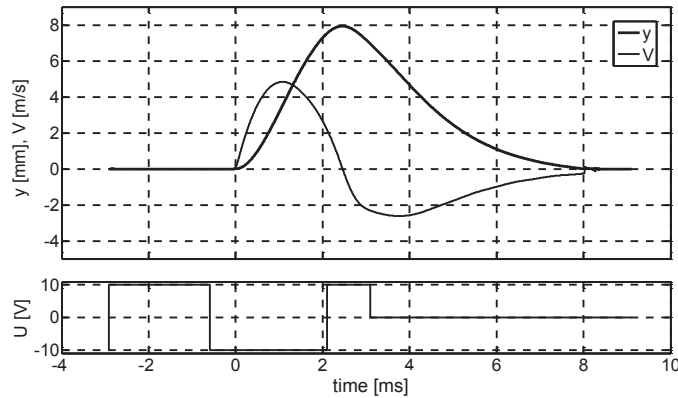
Fig. 9. Waveforms of: valve lift, valve speed and the control signal for a supply pressure of 14 MPa and duration of valve lift 8 ms
