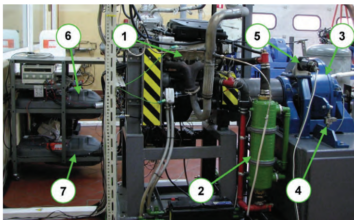
Fig. 3. Test stand – general view: 1 – research engine of Fiat 1100 MPI type, 2 - radiator, 3 – eddy-current engine brake made by Schenck, 4 – transducer of engine load, 5 – engine speed sensor, 6 – alcohol tank, 7 – gasoline tank
