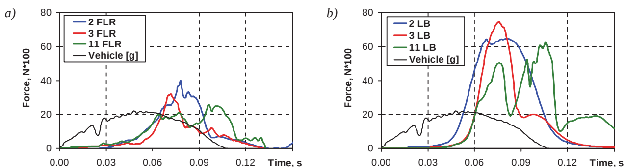
Fig. 6. A course of forces in thighs (FLR) and reactions in the lap belt (LB) in the time function
