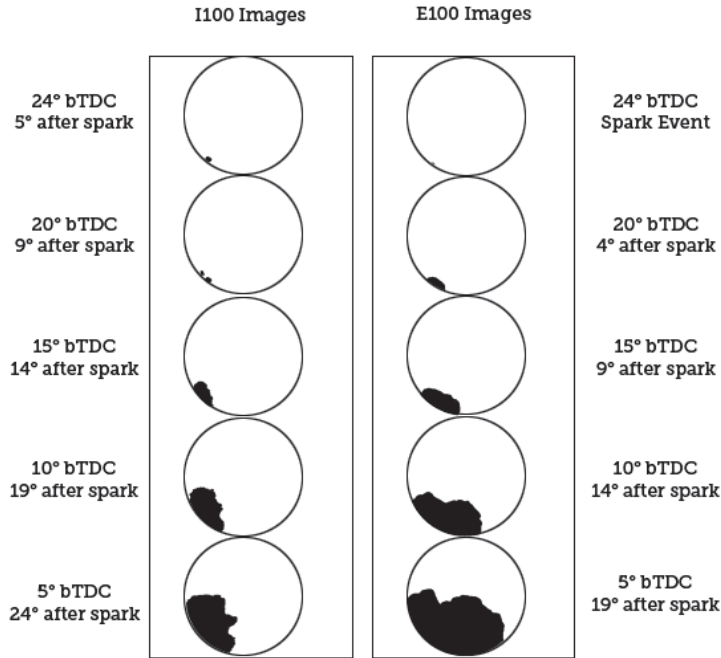
Fig. 5. Side-by-side comparison of the iso-octane (I100) and ethanol (E100) images captured
