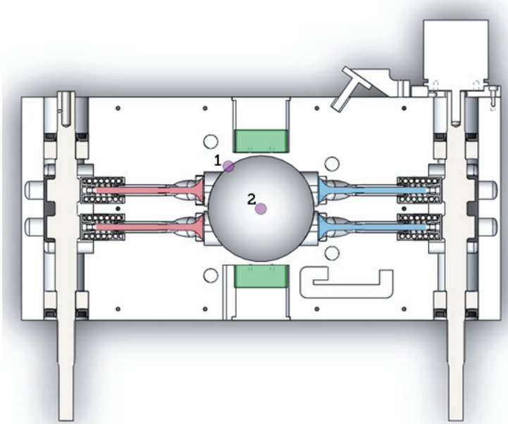
Fig. 1. Overhead view of the redesigned Lister head with the inlet valves shown in blue (right), the exhaust valves shown in red (left), the side windows in green (top and bottom of bore) and the alternative spark locations (1: side and 2: central) as purple discs
