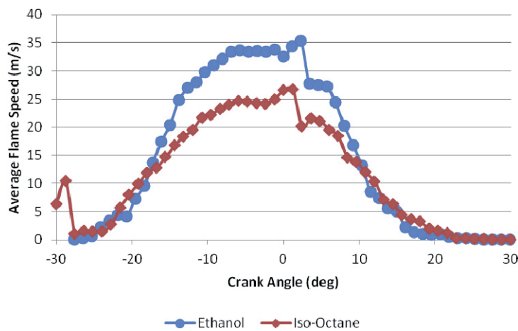
Fig. 6. Flame speed traces for both ethanol and iso-octane fuels
