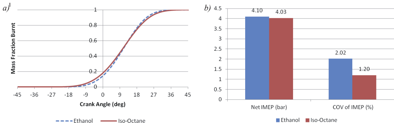
Fig. 4. a) Wiebe function curve and b) IMEP and COV of IMEP
