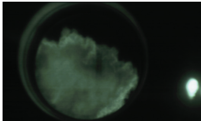
Fig. 2. Graphic detailing a standard image captured during combustion. The bore is evident from the 'halo' of light around it with the propagating flame clear in the centre. The burst of light on the right-hand side is to indicate TDC
