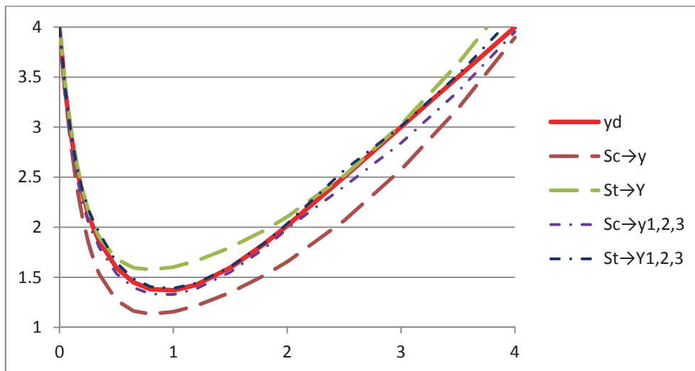
Fig. 2.1. Course exact solution y_d of the equation (2.1), approximate solution y i Y for the interval 1 \leq y \leq 4 , and y_1 i Y_1 , y_2 i Y_2 , y_3 i Y_3 for the intervals 4 \geq y_1 \geq 2 ; 2 \geq y_2 \geq 1.2 ; 2 \leq y_3 \leq 4
