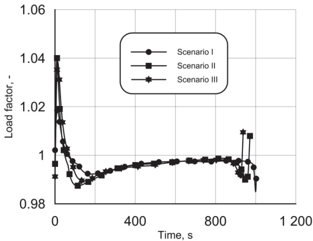
Fig. 5. The optimal change of load factor
