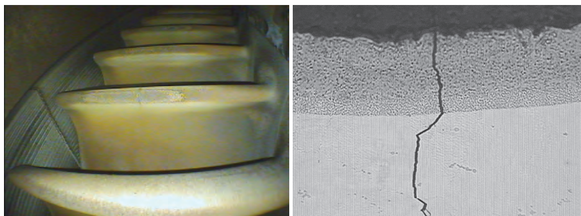
Fig. 1. Image of a crack of the protective coating with crack propagation into the parent material of the blade body [5]: videoscopic image – a) microscopic image, magn. \times 450
