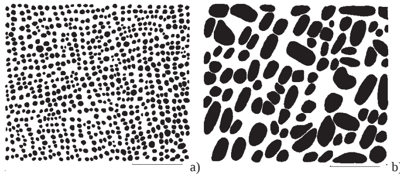
Fig. 6. The microstructure of turbine blades after heating at temperatures: a) - 1123 K, b) - 1423 K (magn. \times 20000 ) – one can see coagulation, alteration of shapes and corrugation of the \gamma' phase formations.
