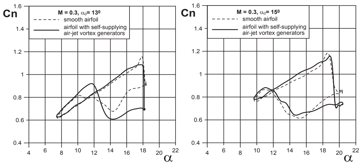
Fig. 6. Influence of the self-supplying AJVGs on normal force coefficient at M = 0.3 and \alpha_0 = 13.15^\circ
