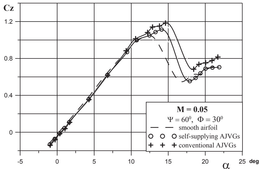
Fig. 5. Comparison of the lift coefficient vs. angle of attack for the conventional and self-supplying AJVGs
