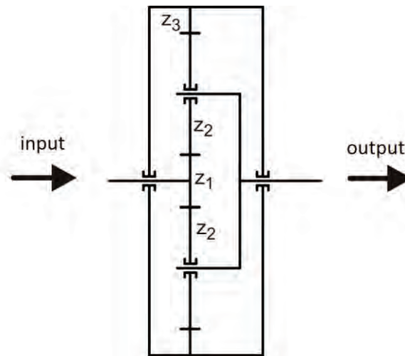
Fig. 1. A diagram of power transmission of the tested planetary gearing
