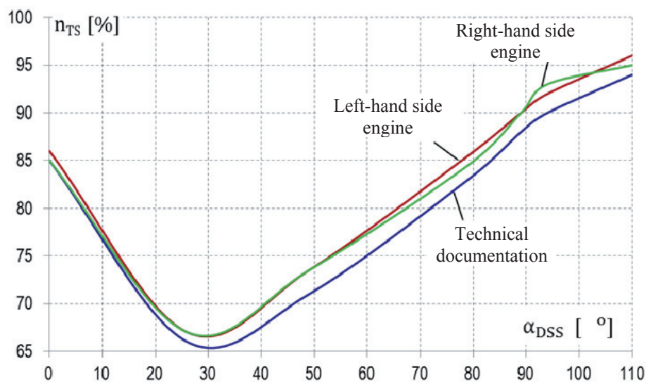
Fig. 1. Relationships between turbocompressor rpm for the right-hand side and left-hand side engines and the tilt angle of the Engine Control Lever (DSS)
