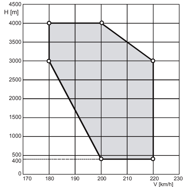
Fig. 6. The enveloped of engine start-ups plotted for the Bryza-1R aircraft with the TWD-10B/PZL-10S engine furnished with the HC-B5MP-3D/M airscrew from Hartzell
