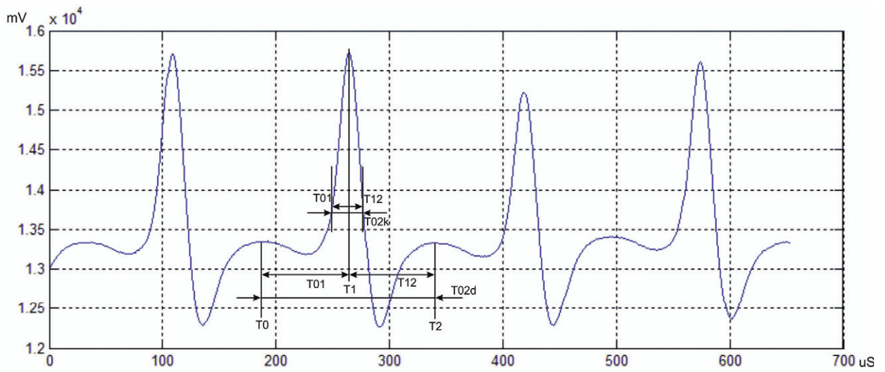
Fig. 2. Signal from induction sensor
