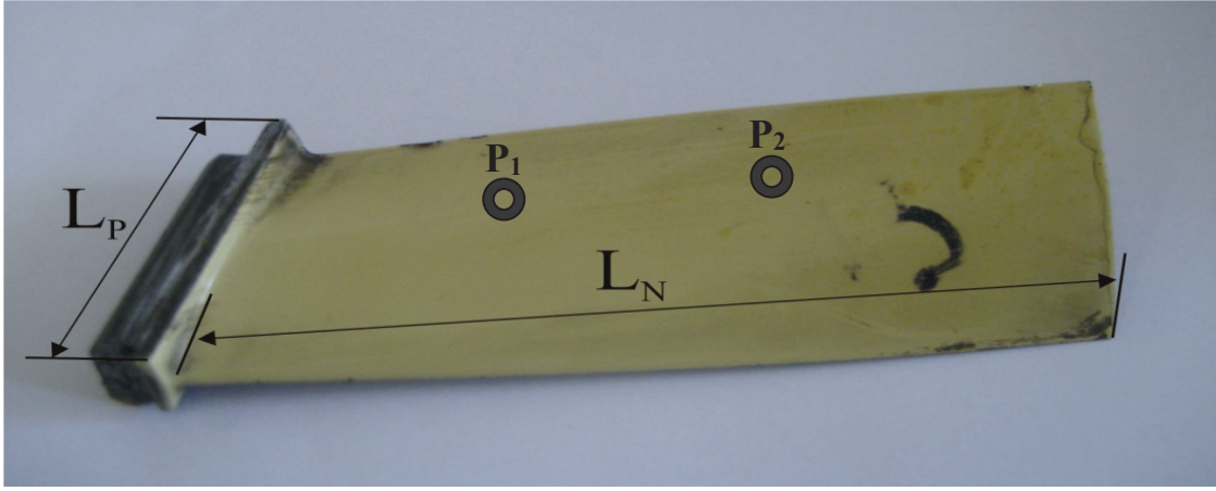
Fig. 1. First grade blade of axial compressor of aircraft engine SO-3 L_N=113 mm, L_p=40 mm with indicated points of oscillation inductor
