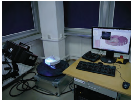
Fig. 1. Measuring the gear wheel for aeronautical dual-power path gearing by means of optical 3D scanner ATOS II TripleScan
