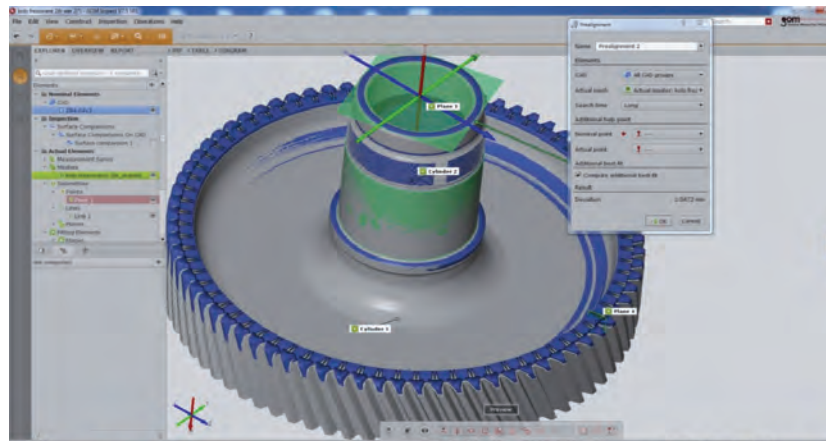
Fig. 4. Combining the CAD model with the surface model of the measured gear after the coordinate system is eventually defined
