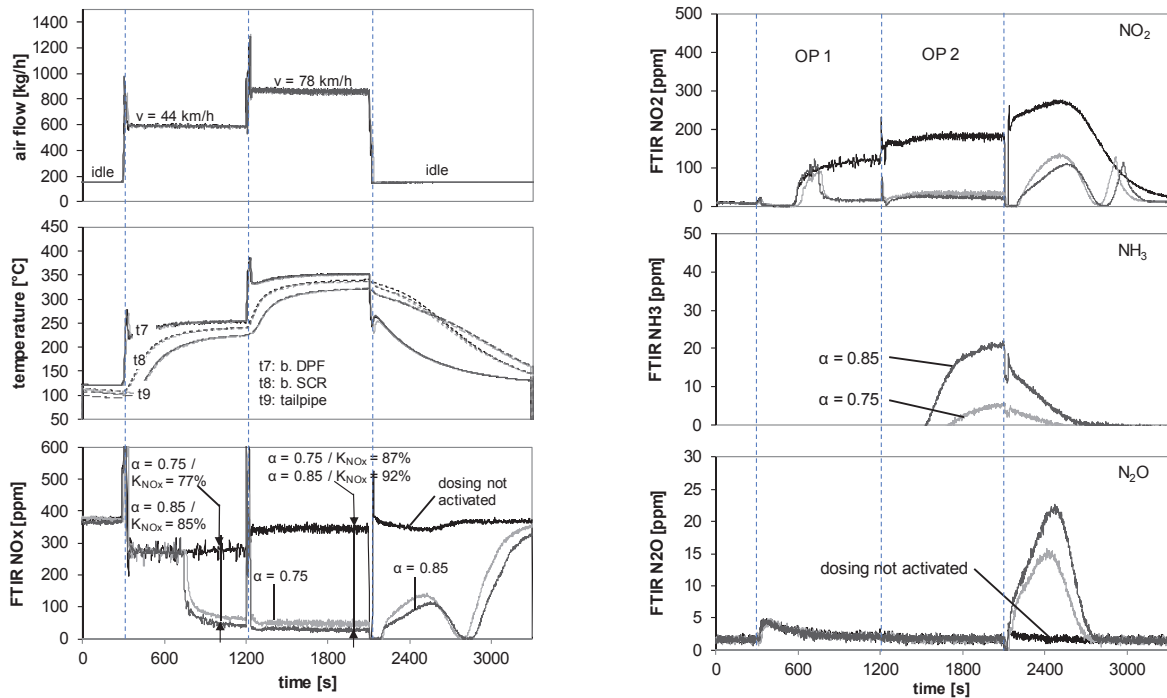
Fig. 1. Step test with different dosing rate after 1000h, retrofit system cDPF and SCR, dosing: not activated / 0.75 / 0.85 vehicle A, ULSD, chassis dyno
