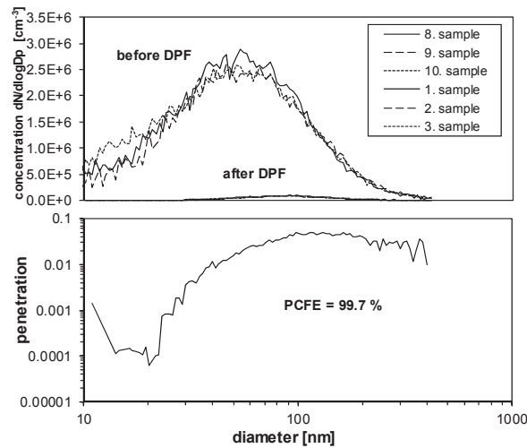
Fig. 2. SMPS size spectra at OP2 and NP-filtration of a retrofitted DPF. OEM SCR, dosing activated, vehicle E, chassis dyno MAN
