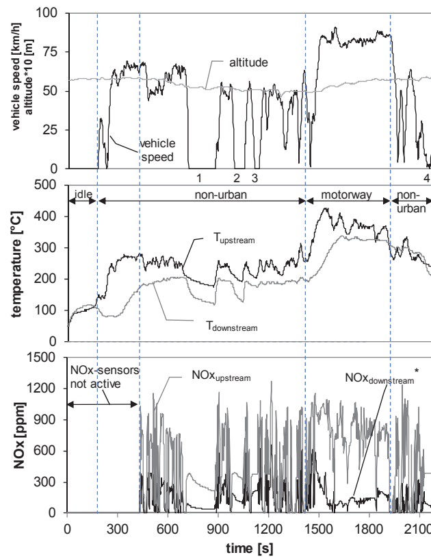
Fig. 4. Hybrid on road trip – switching off the engine. Vehicle B CRT & SCR, ULSD, AdBlue. 1) railroad crossing – combustion engine off, 2) traffic light – combustion engine off, 3) traffic light – combustion engine on, 4) reverse – combustion engine off. * NO x downstream values from NO x -sensor, without consideration of the cross-sensitivity
