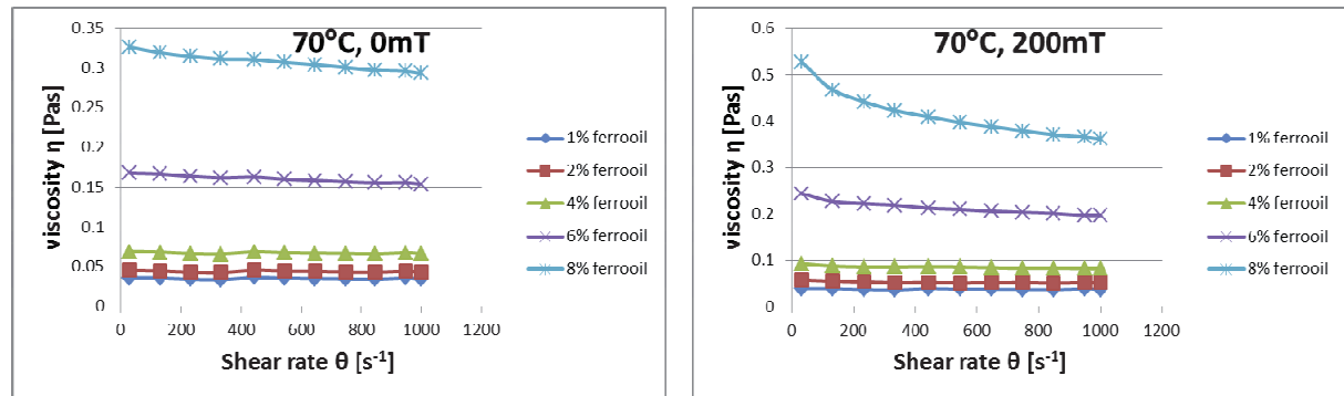
Fig. 3. Characteristics of a dynamic viscosity of 1%, 2%, 4% 6% and 8% ferro-oils for magnetic induction field B=0\text{mT} and B=200\text{mT} in terms of changes in the shear rate range 0-1000 \text{s}^{-1} for the temperature t=70^\circ\text{C}
