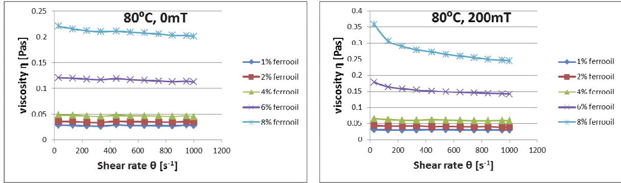
Fig. 4. Characteristics of a dynamic viscosity of 1%, 2%, 4% 6% and 8% ferro-oils for magnetic induction field B=0\text{mT} and B=200\text{mT} in terms of changes in the shear rate range 0-1000 s-1 for the temperature t=80^\circ\text{C}
