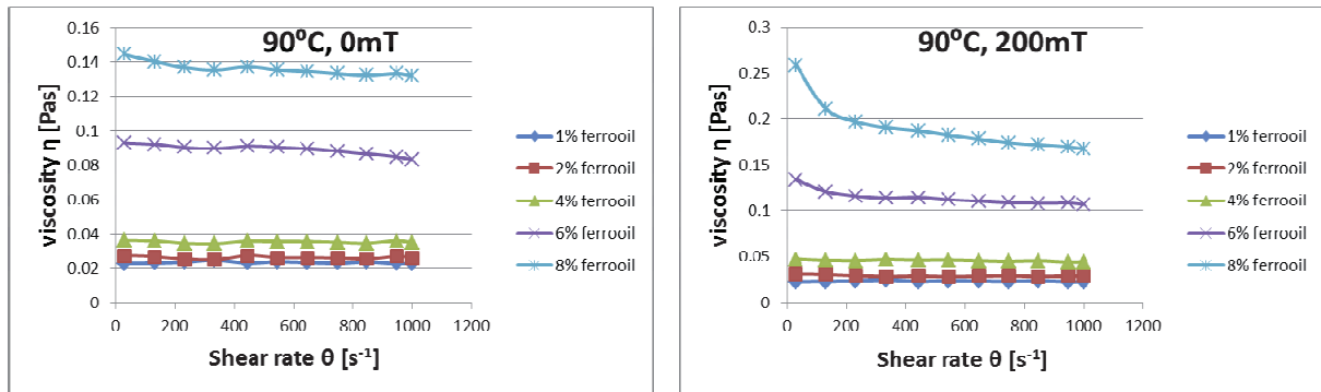
Fig. 5. Characteristics of a dynamic viscosity of 1%, 2%, 4% 6% and 8% ferro-oils for magnetic induction field B=0\text{mT} and B=200\text{mT} in terms of changes in the shear rate range 0-1000 s-1 for the temperature t=90^\circ\text{C}
