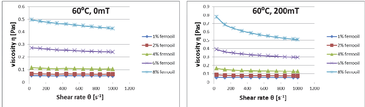
Fig. 2. Characteristics of a dynamic viscosity of 1%, 2%, 4% 6% and 8% ferro-oils for magnetic induction field B=0\text{mT} and B=200\text{mT} in terms of changes in the shear rate range 0-1000 \text{s}^{-1} for the temperature t=60^\circ\text{C}
