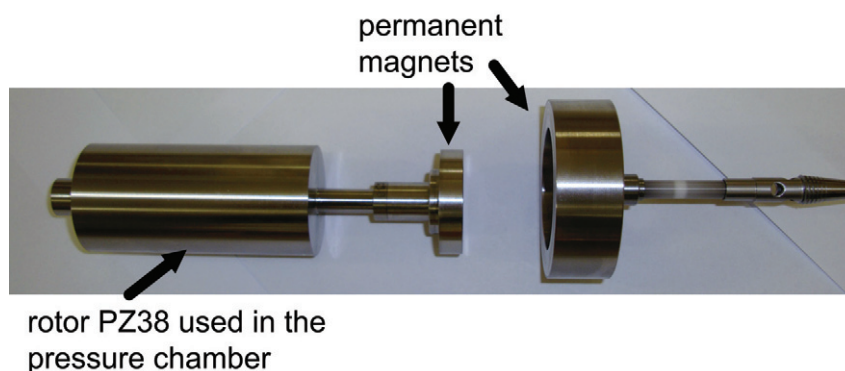
Fig. 2. The rotor PZ38 used for measurements in the pressure chamber
