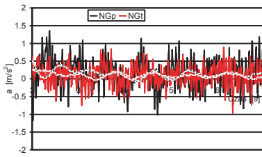
Fig. 6. Time histories of the head accelerations: test drives on the road section with "even" (asphalt) surface (A, cases NGp and NGt)
