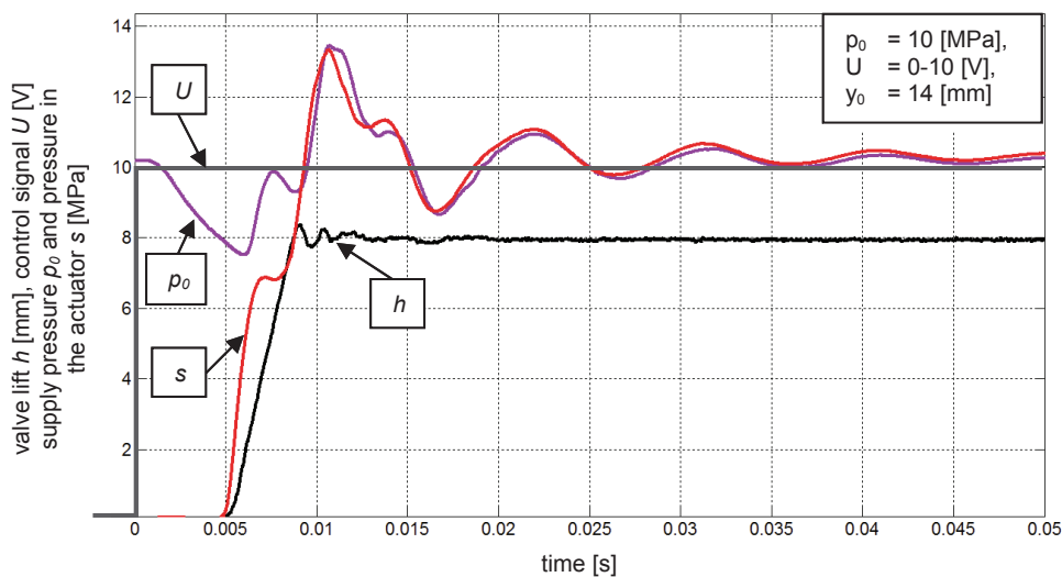
Fig. 4. Waveforms of: valve lift “ h ”, the supply pressure “ p_0 ” control signal “ U ”, the pressure in the actuator “ s ” for step control signal of value 10 V, the supply pressure equal 10 MPa and the valve spring deflection “ y_0 ” equal 14 mm
