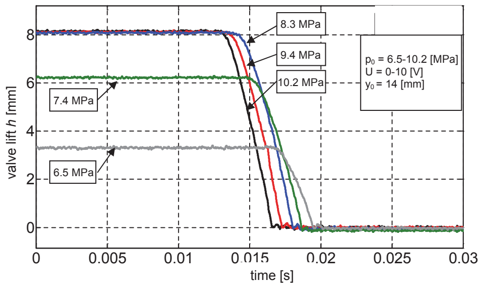
Fig. 8. Influence of supply pressure on waveforms of valve closing for bipolar signal
