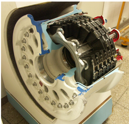
Fig. 3. Multi-disc aviation brake. (source: Internet)
