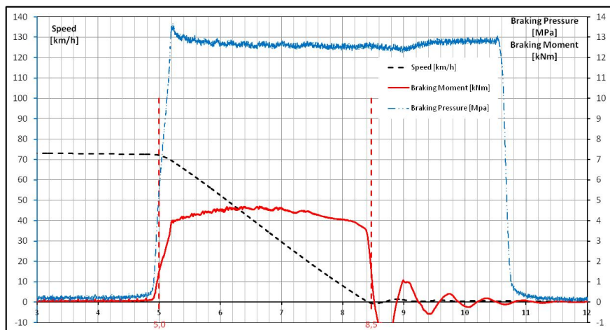
Fig. 11. Model (friction material) test of the automotive brake – IL68 Test Stand
