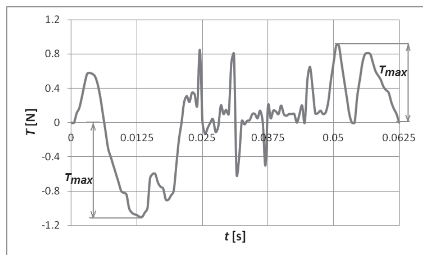
Fig. 6. Measured values of friction force T between valve and its guide vs. time t : loading frequency f = 16 Hz, maximum valve lift h_{\max} = 5 mm, T_{\max} – maximum friction force during valve displacement against its guide
